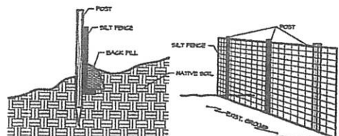
SILT FENCE DETAIL
