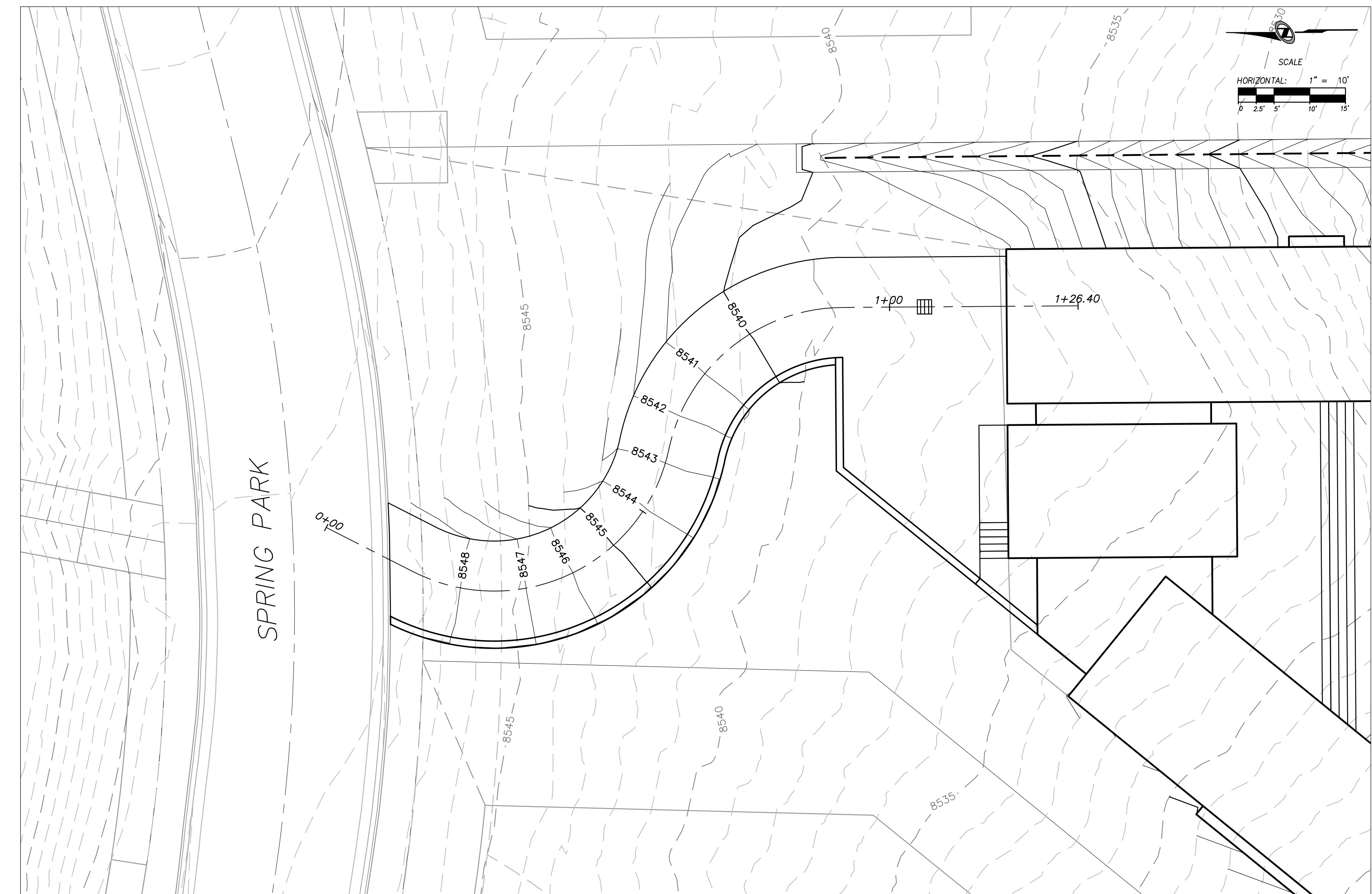
DRIVEWAY PLAN VIEW
