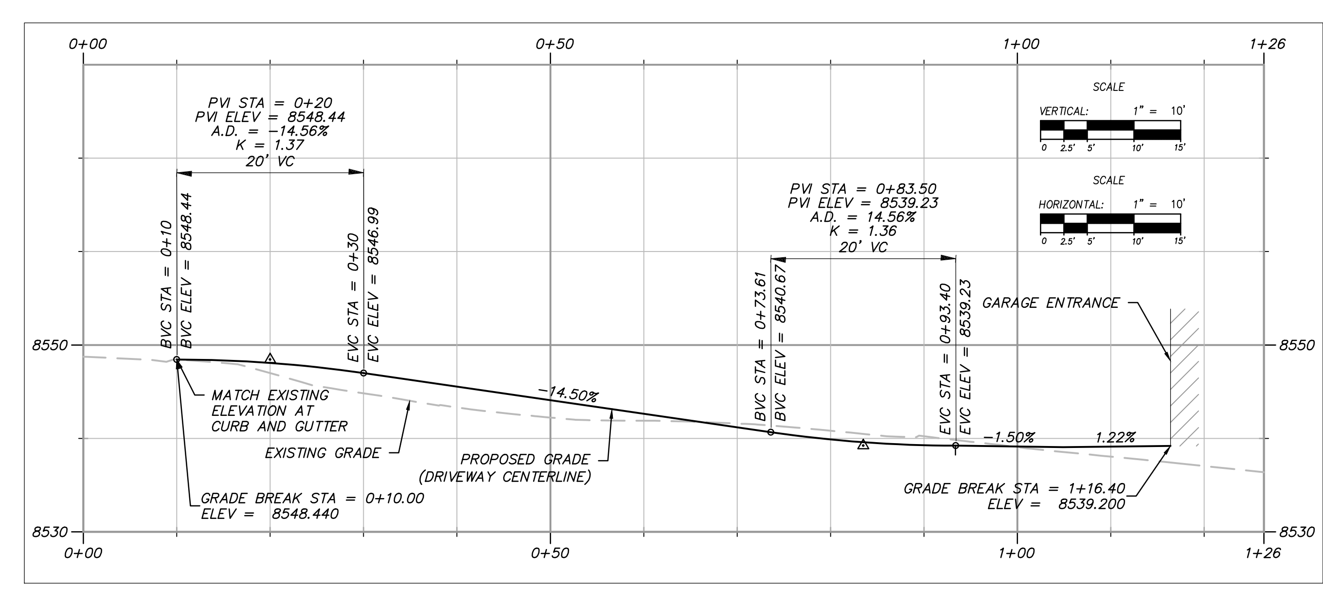
DRIVEWAY PROFILE
