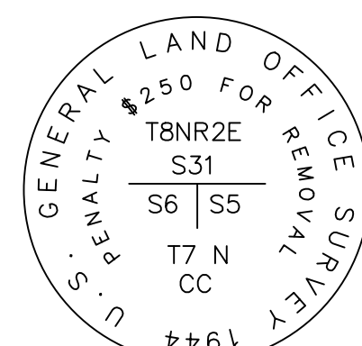
DETAIL "D"
