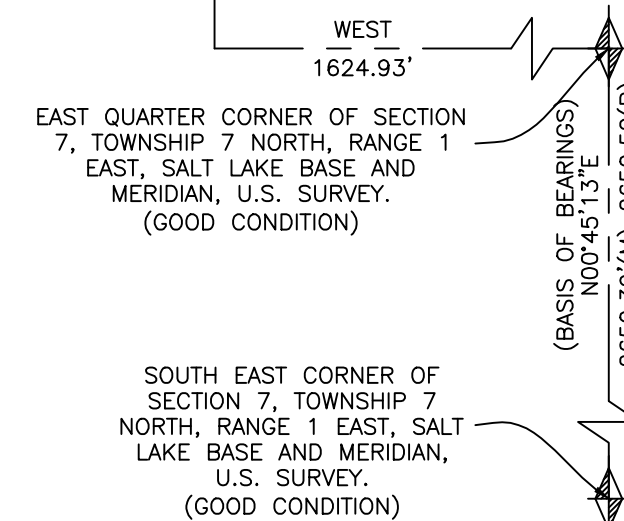
Monument Detail 1 (NOT TO SCALE) Monument Detail 2 (NOT TO SCALE)
