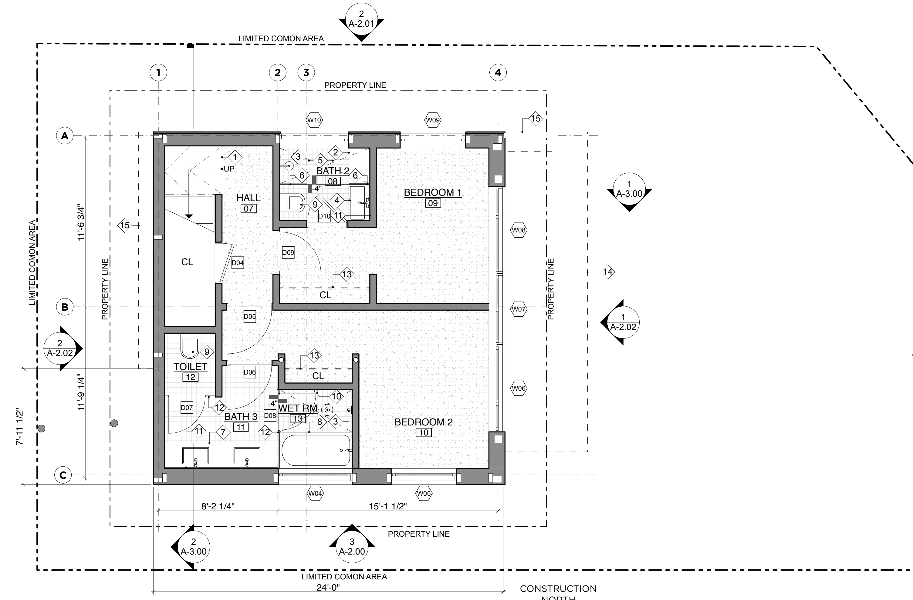
FIRST FLOOR PLAN SCALE: 1/4" = 1'-0" 1
