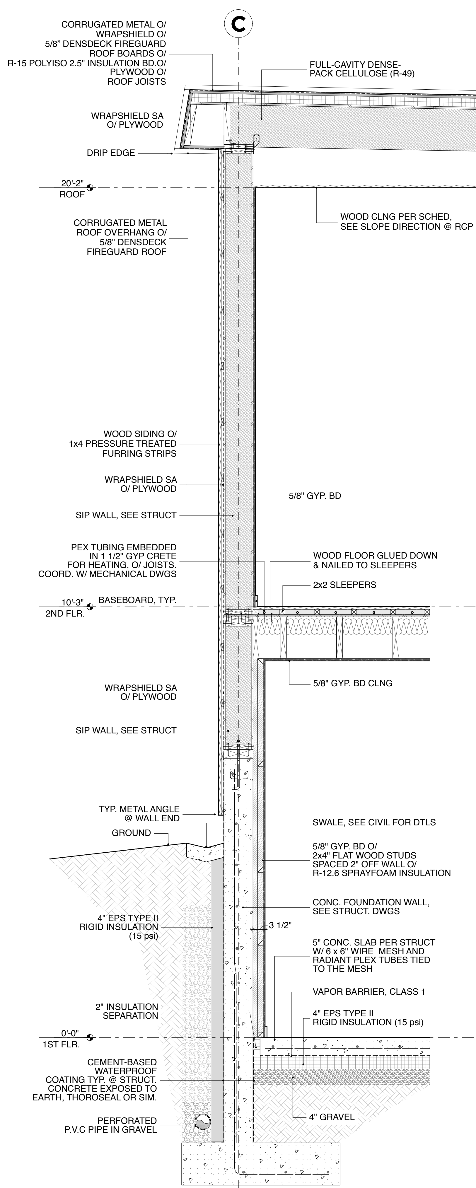
WOOD WALL SECTION 4 SCALE: 3/4" = 1'-0"
