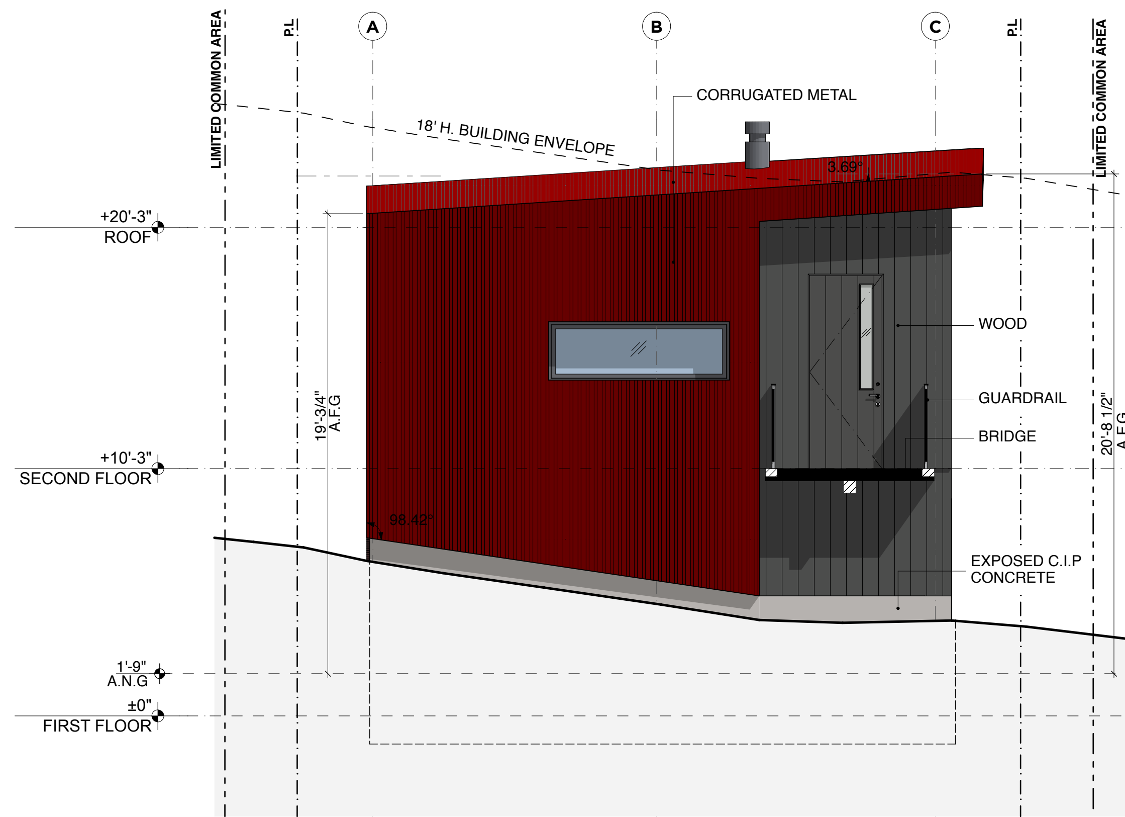
WEST ELEVATION
