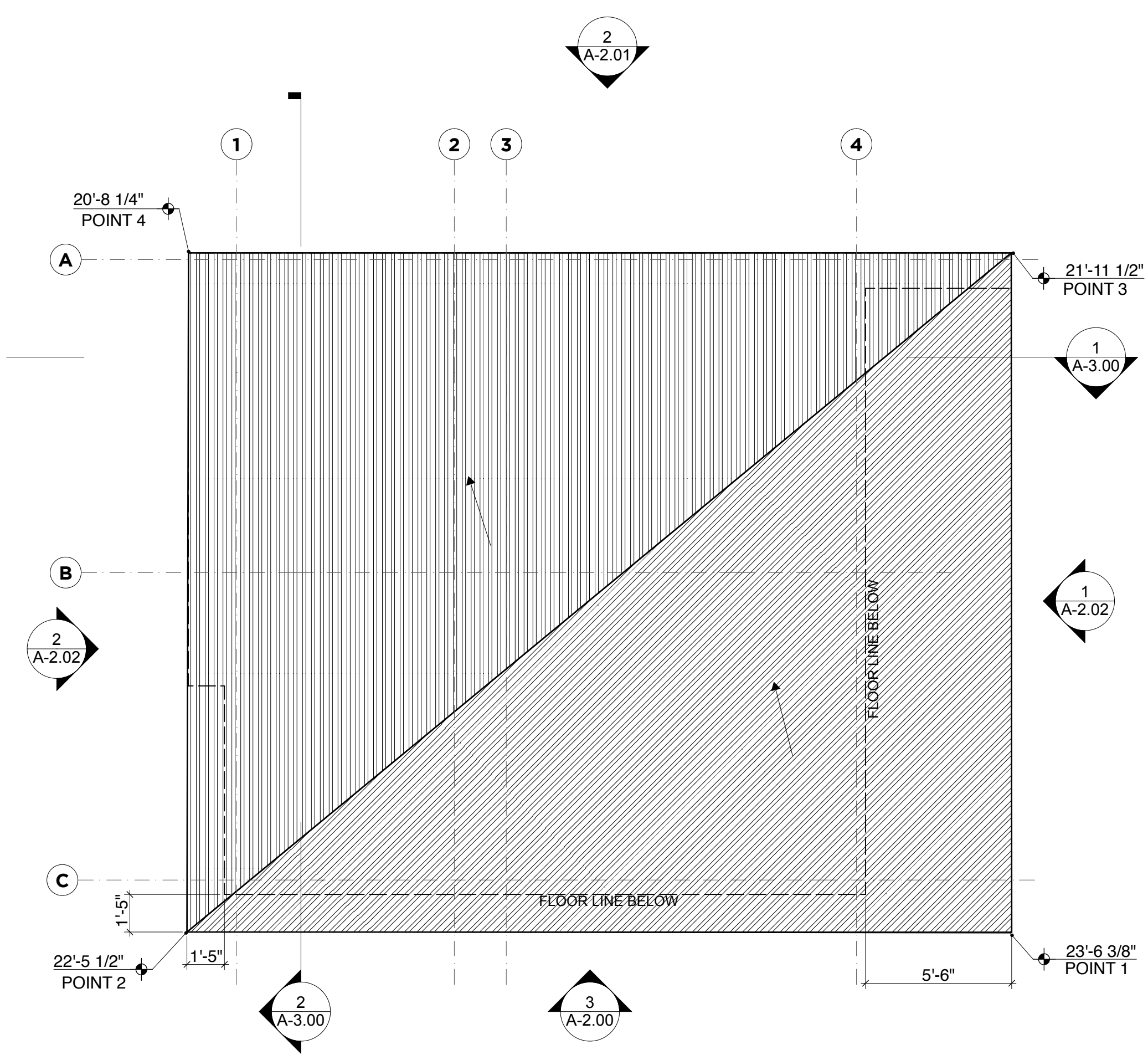
ROOF PLAN SCALE: 1/4" = 1'-0" 3
