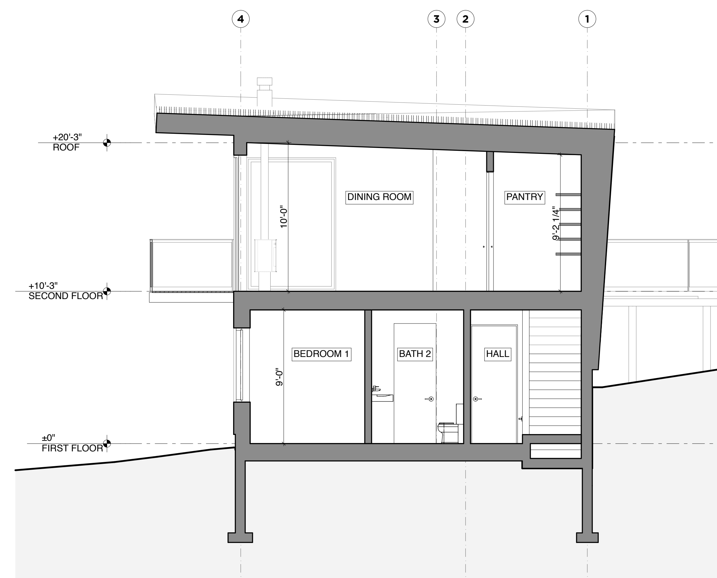
ENTRY SECTION 1 SCALE: 1/4" = 1'-0"
