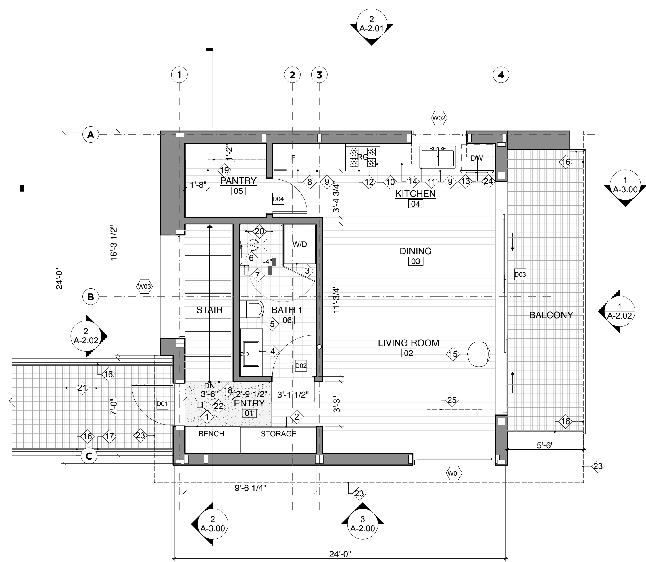
SECOND FLOOR PLAN SCALE: 1/4" = 1'-0" 2
