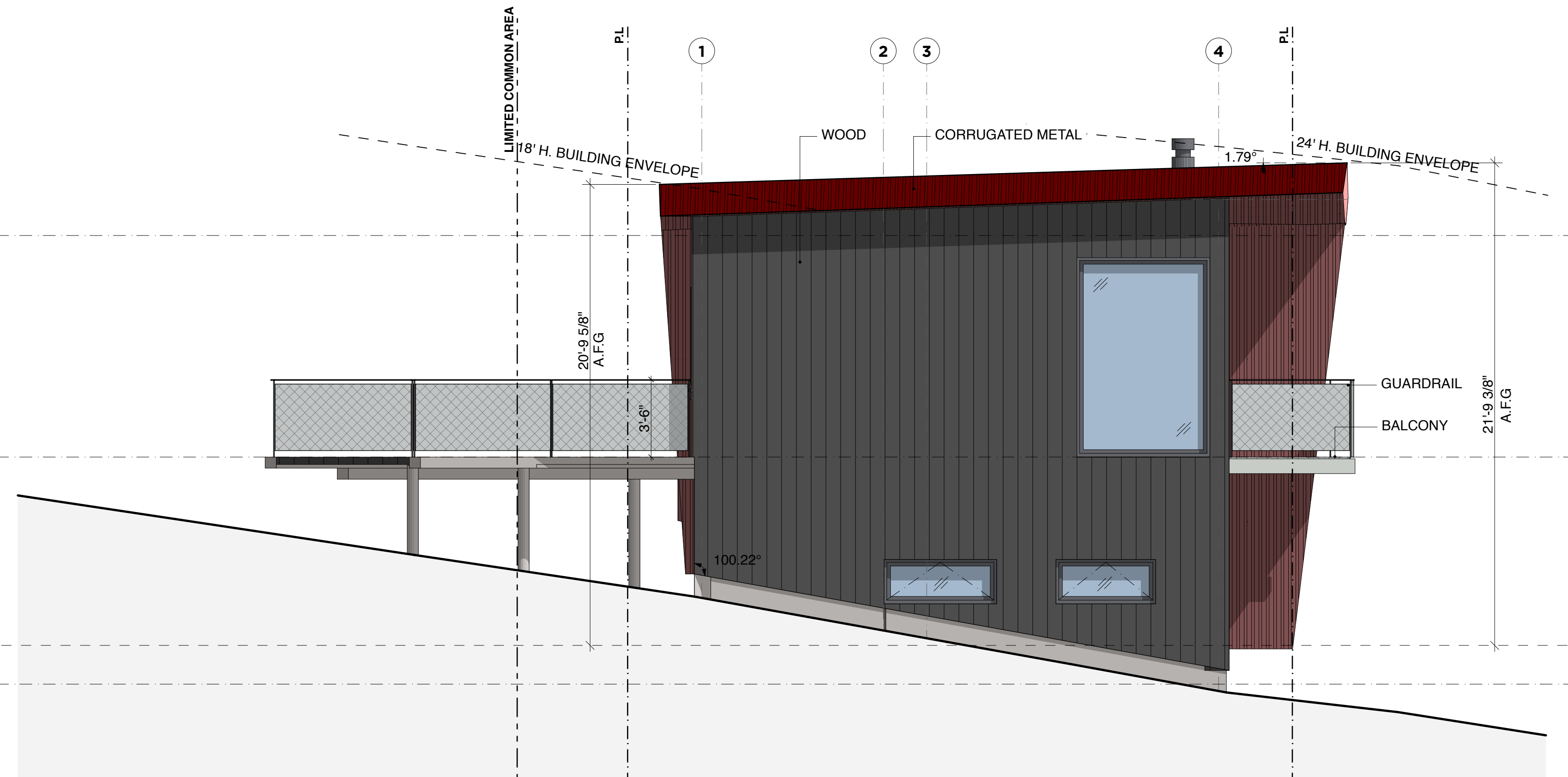
SOUTH ELEVATION
