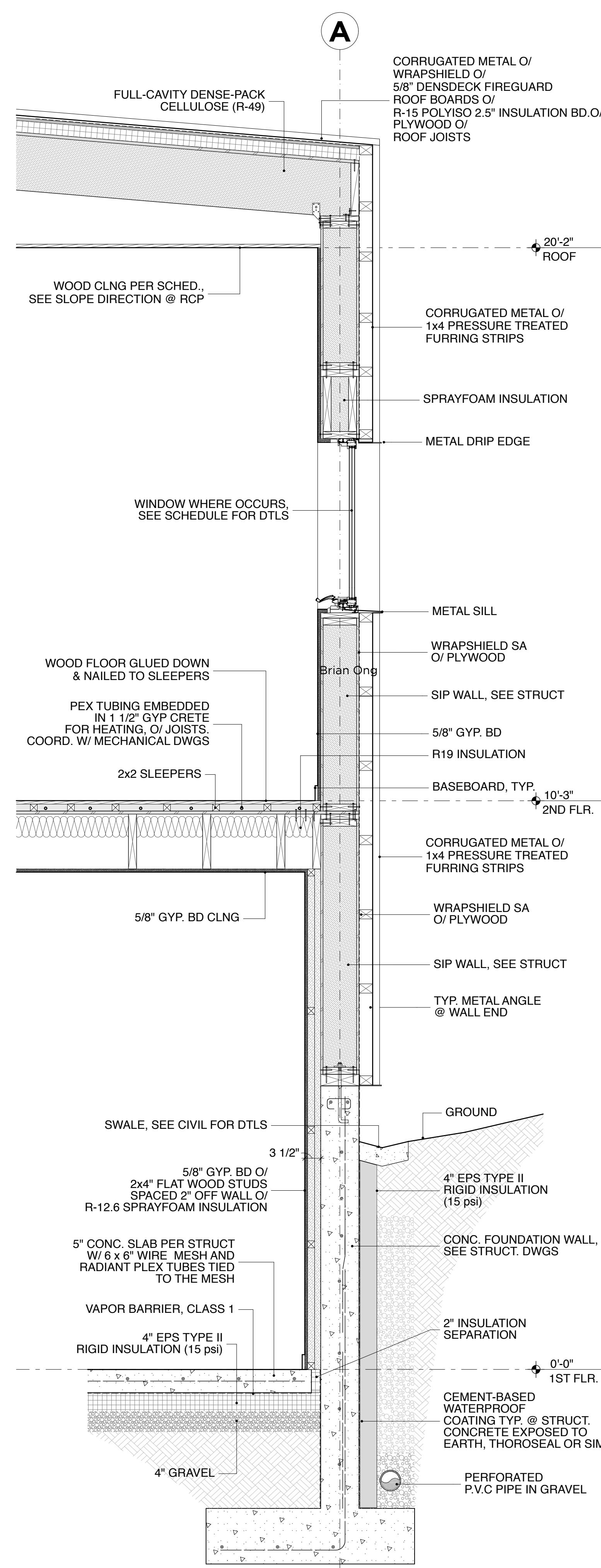
METAL WALL SECTION 3 SCALE: 3/4" = 1'-0"
