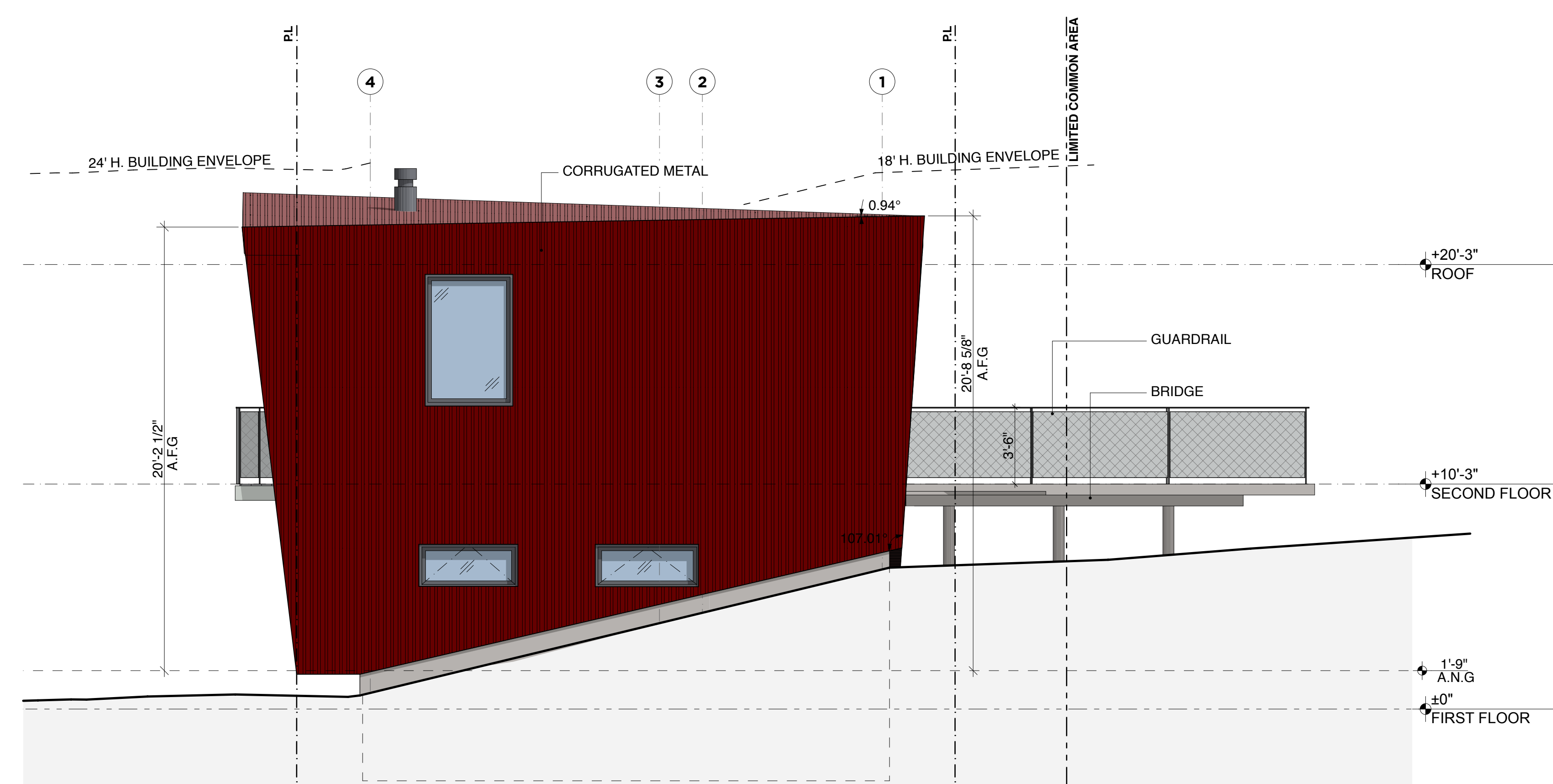
NORTH ELEVATION
