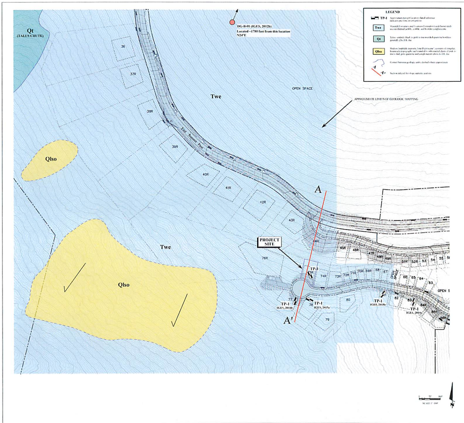
LOCAL GEOLOGY AND GEOTECHNICAL MAP
