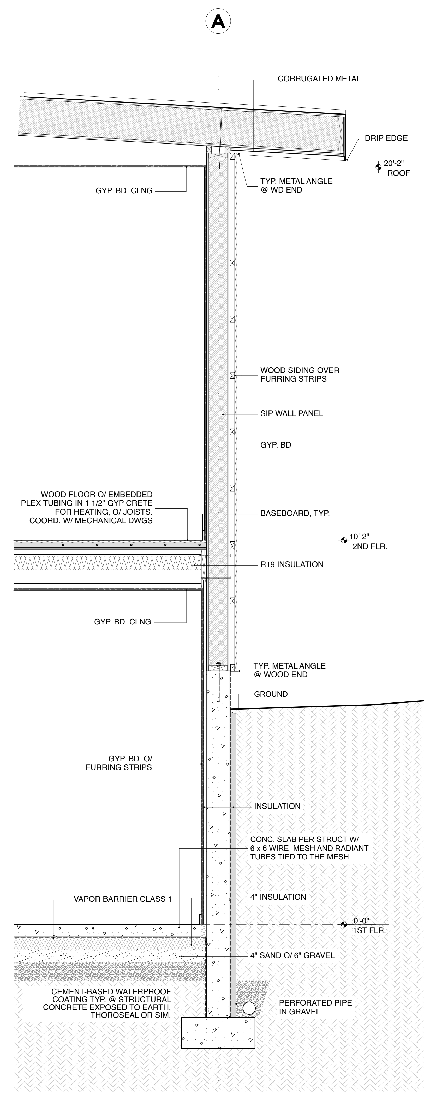
WOOD WALL SECTION SCALE: 3/4" = 1'-0" 3
