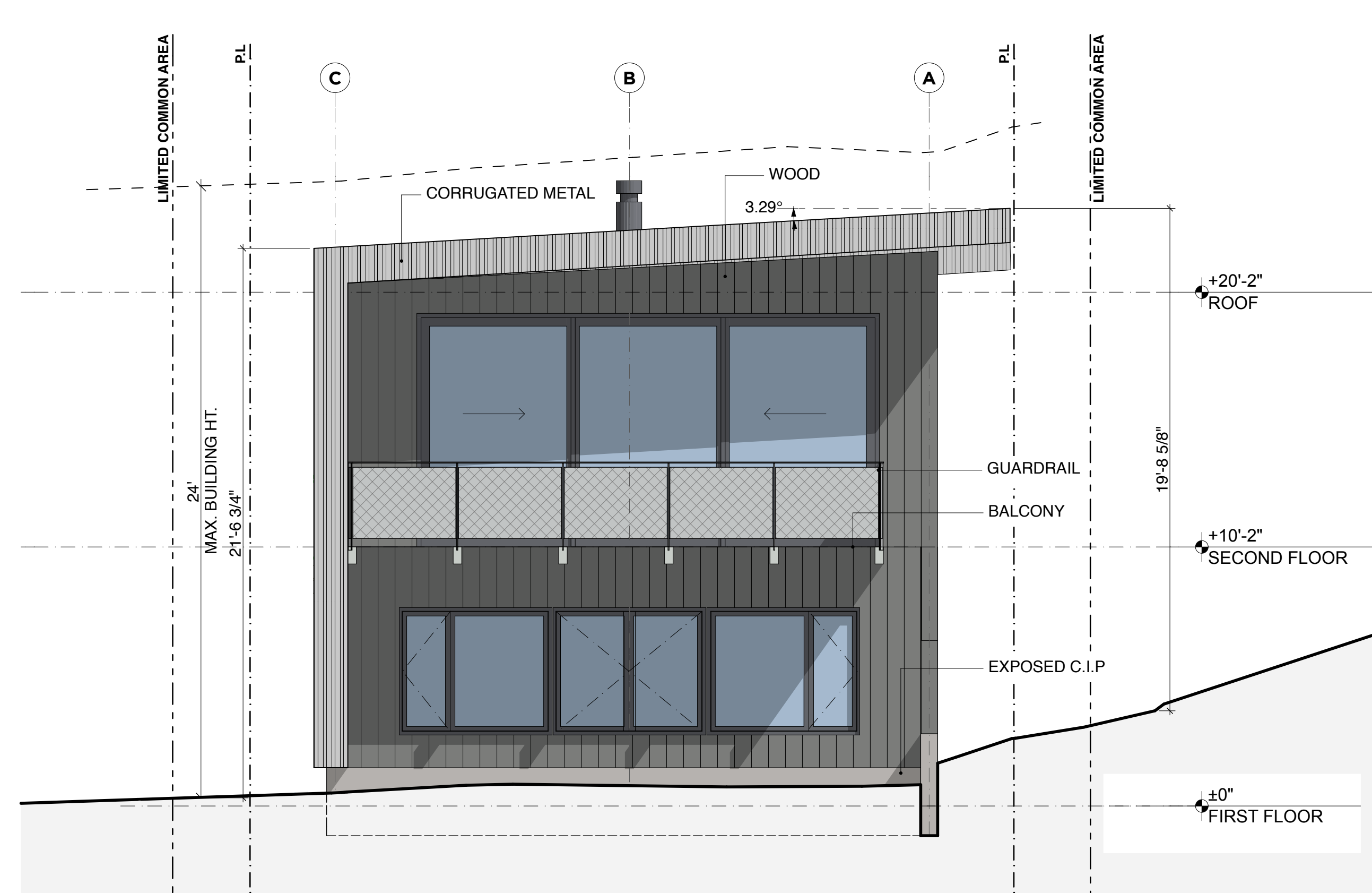
EAST ELEVATION SCALE: 1/4" = 1'-0"
