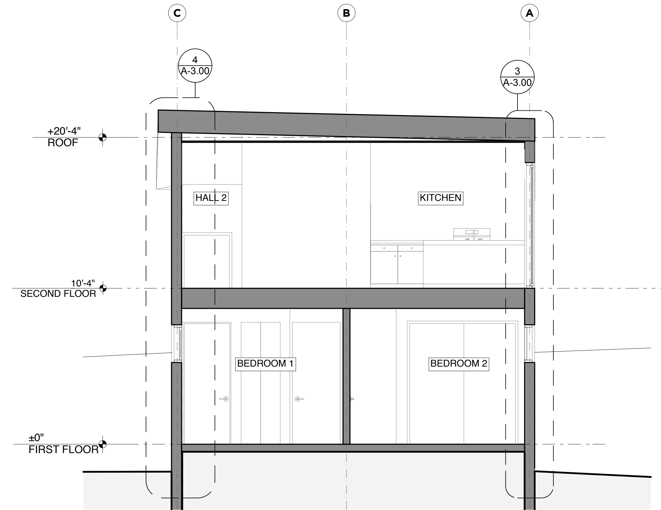
N-S SECTION
