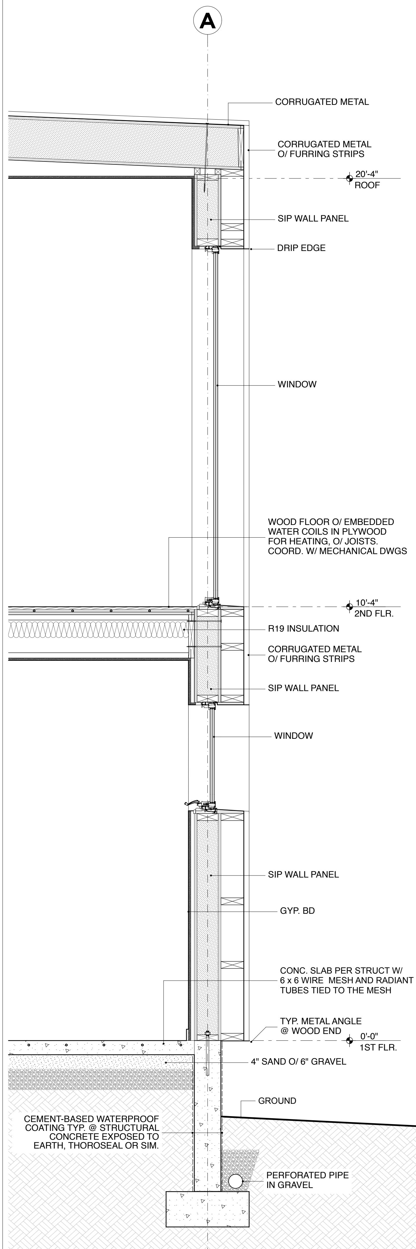
METAL WALL SECTION
