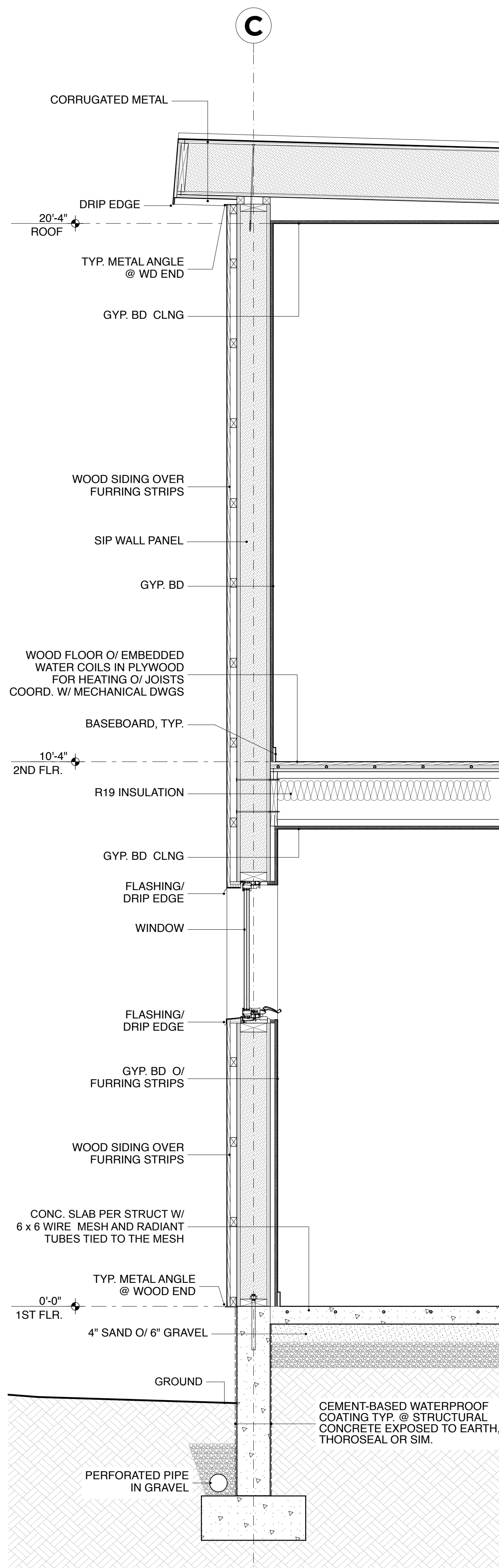
WOOD WALL SECTION
