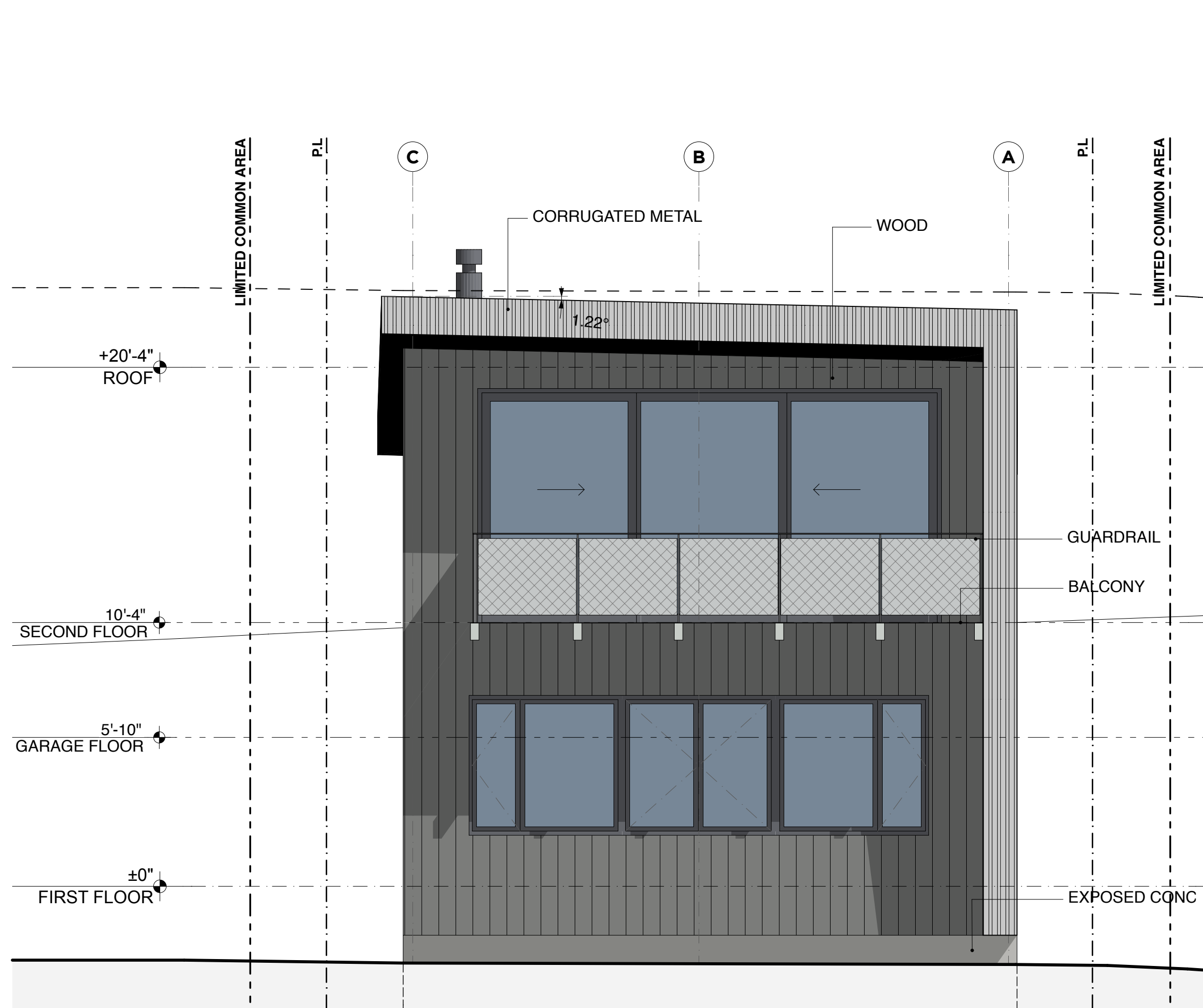
EAST ELEVATION
