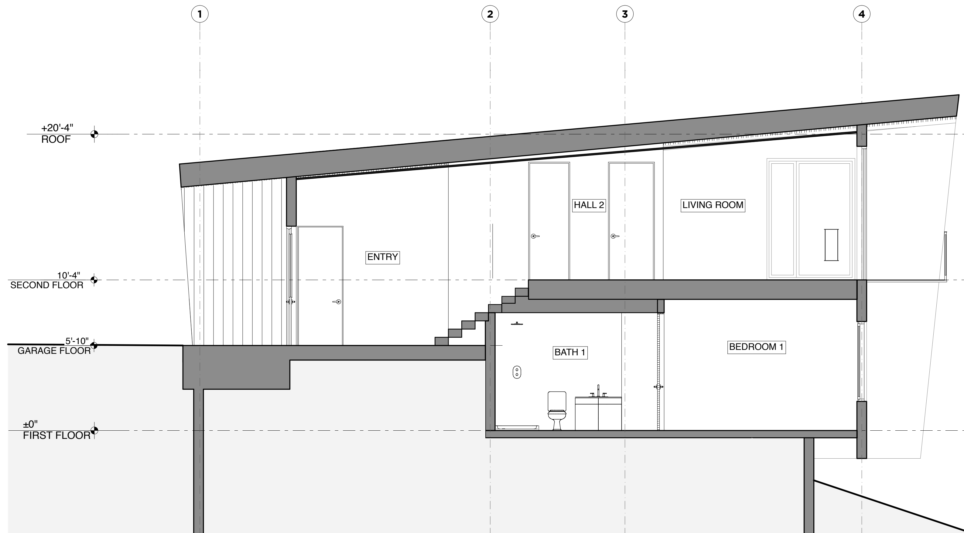
E-W SECTION
