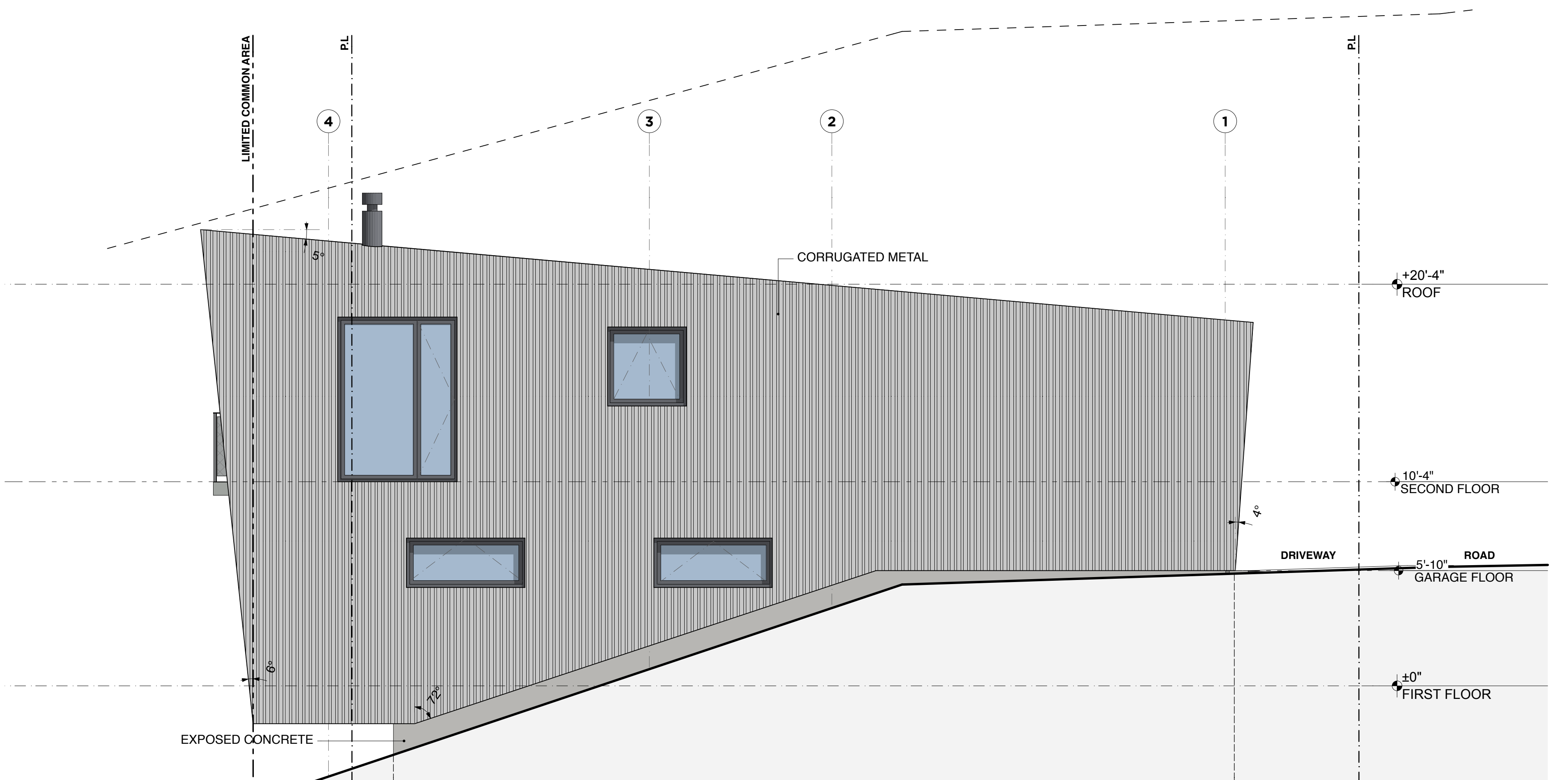
NORTH ELEVATION
