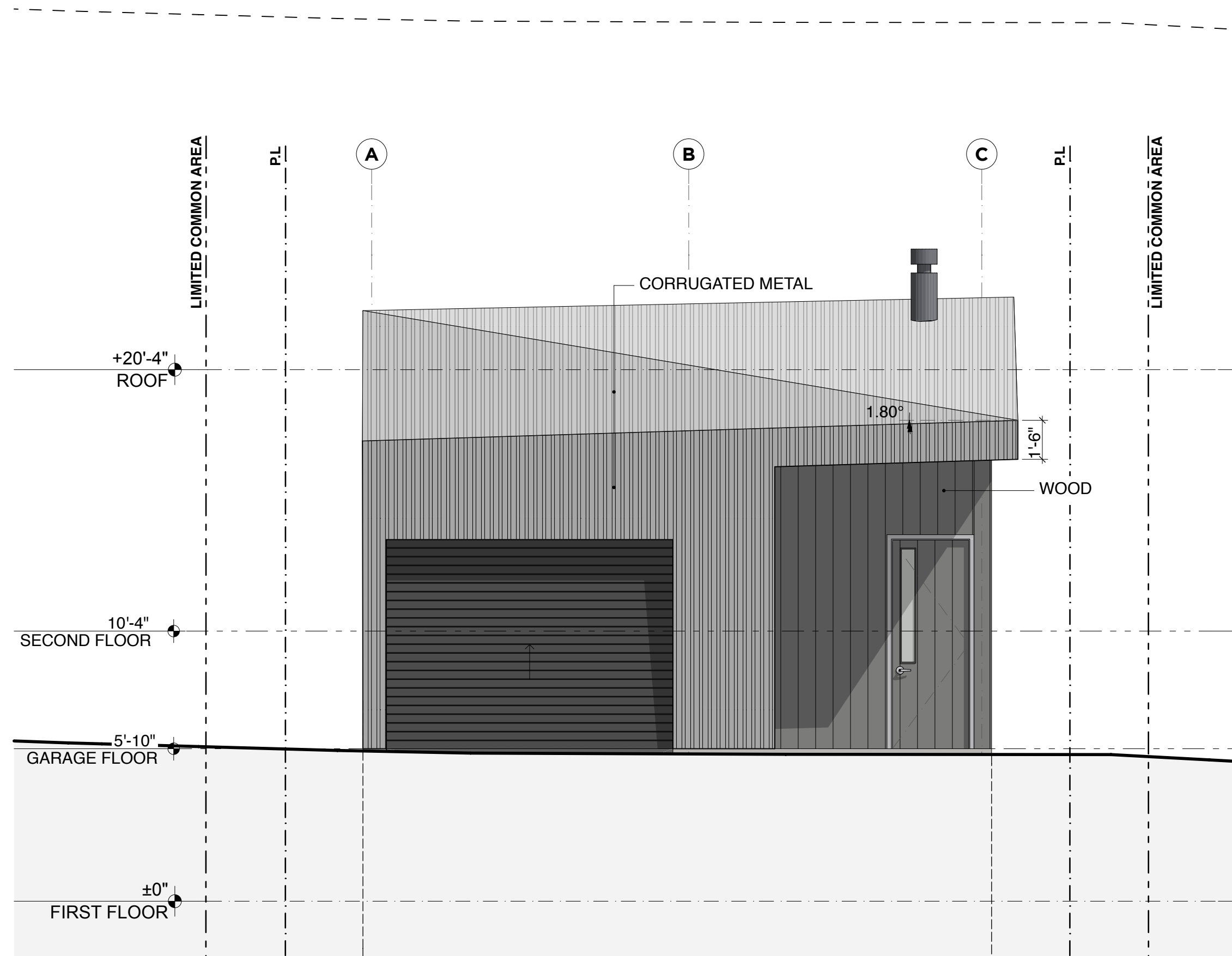
WEST ELEVATION
