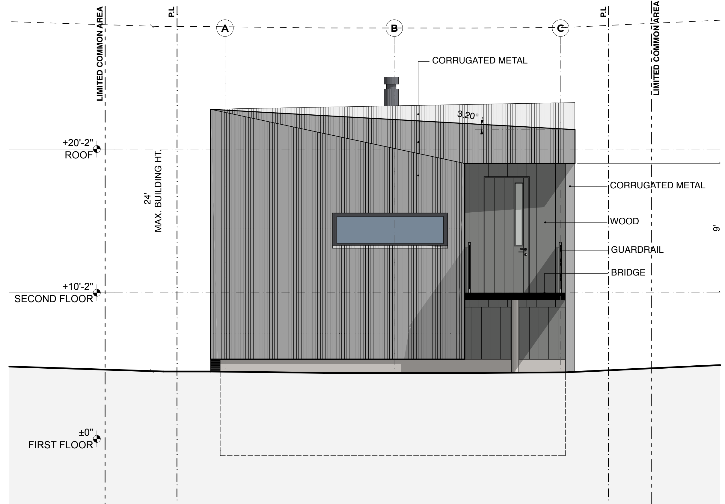
WEST ELEVATION SCALE: 1/4" = 1'-0" ④
