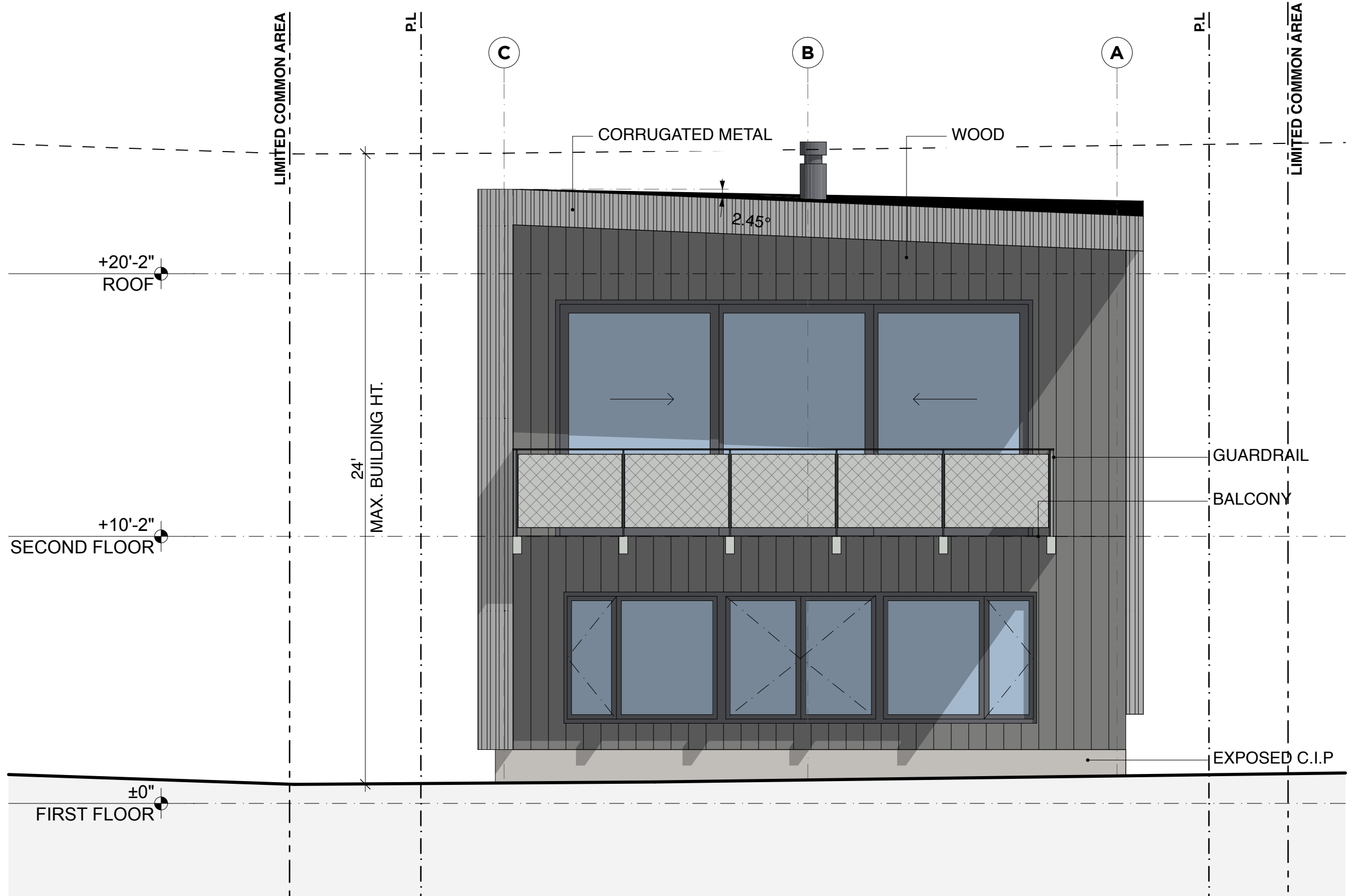
EAST ELEVATION SCALE: 1/4" = 1'-0" ②
