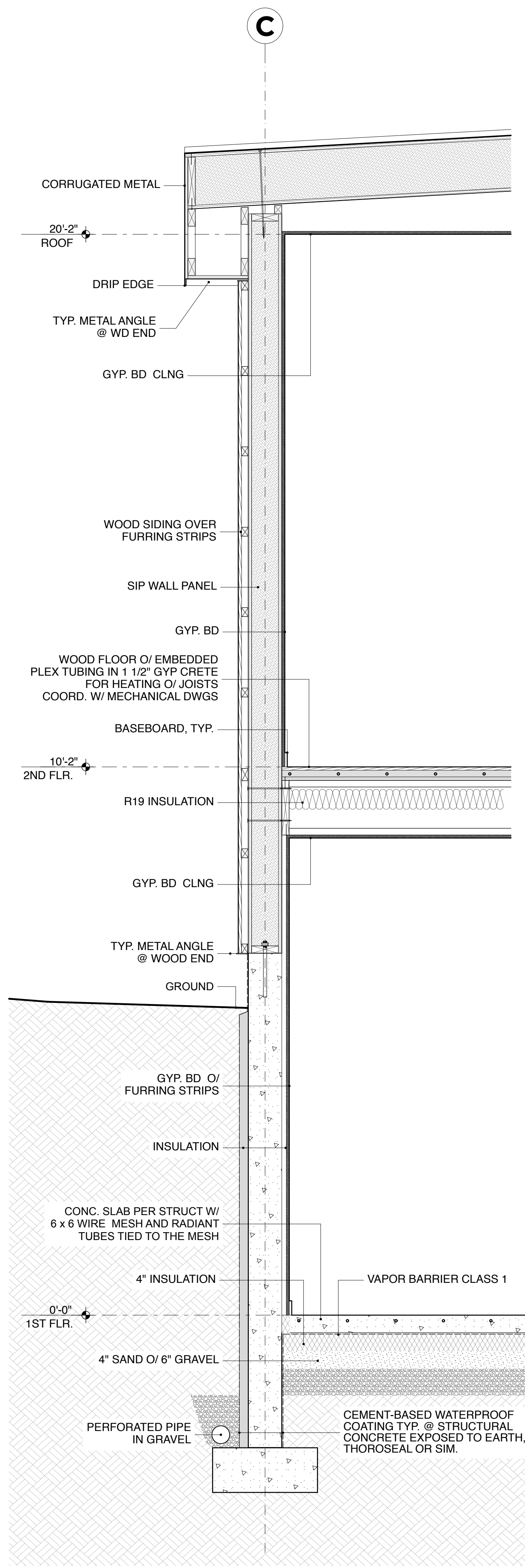
WOOD WALL SECTION SCALE: 3/4" = 1'-0"
