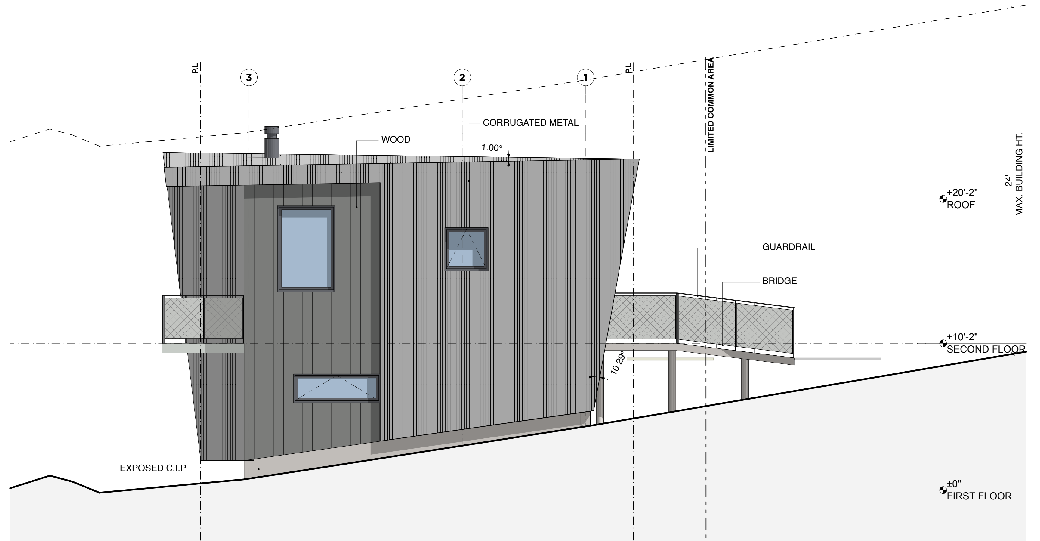
NORTH ELEVATION SCALE: 1/4" = 1'-0" ①
