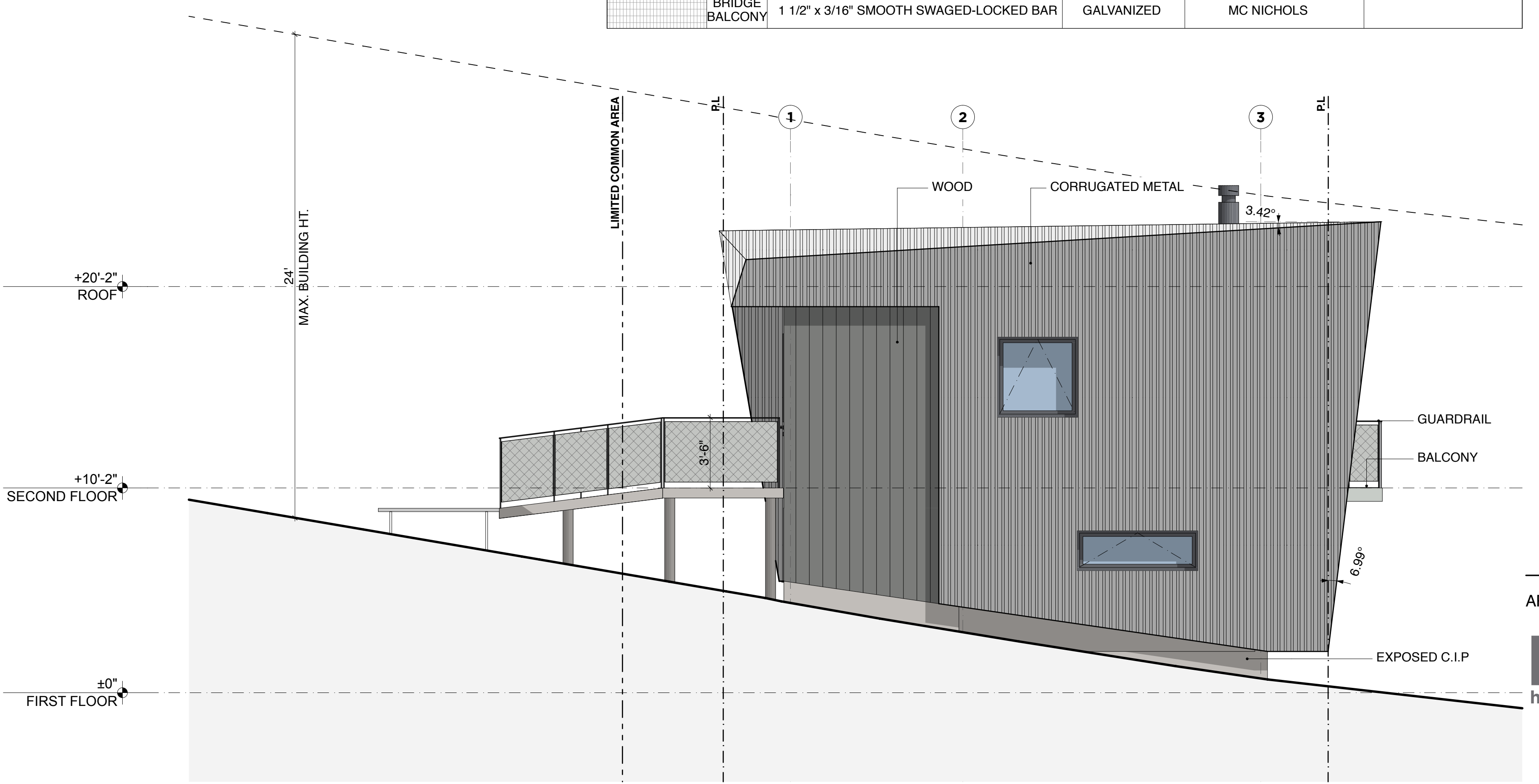
SOUTH ELEVATION SCALE: 1/4" = 1'-0" ③
