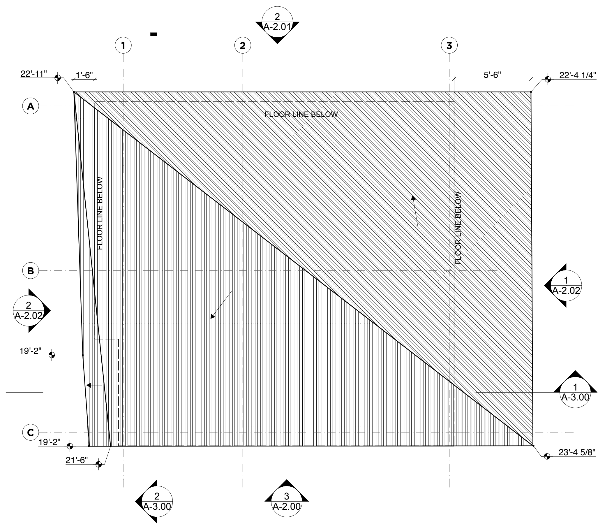
ROOF PLAN
