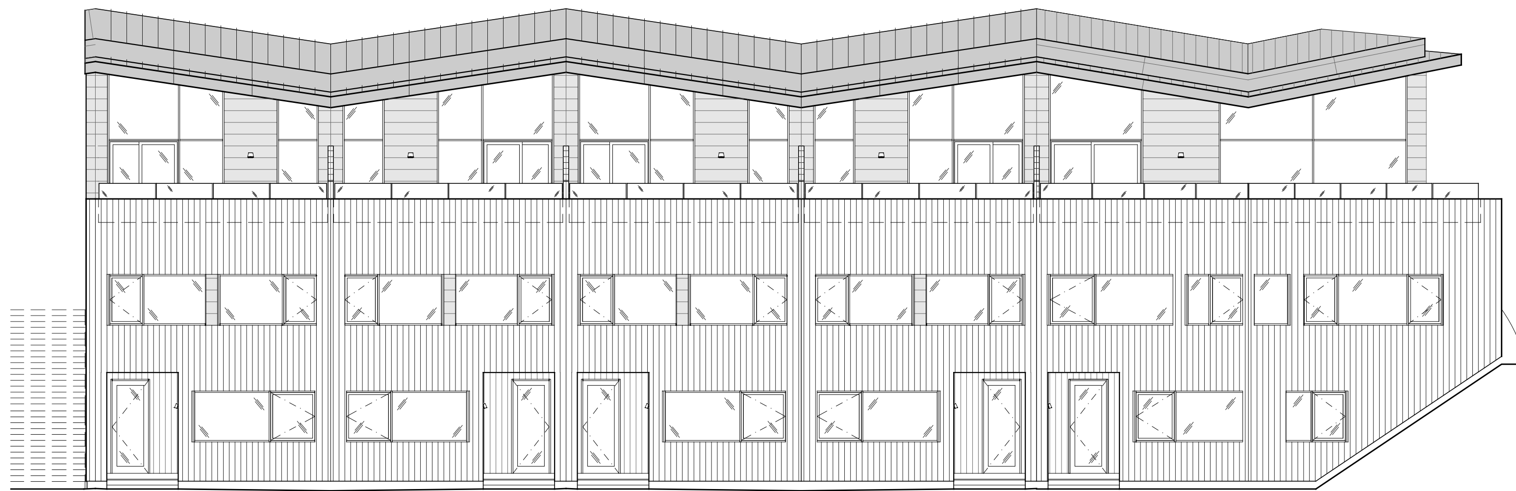
2 OVERALL BUILDING ELEVATION_WEST
