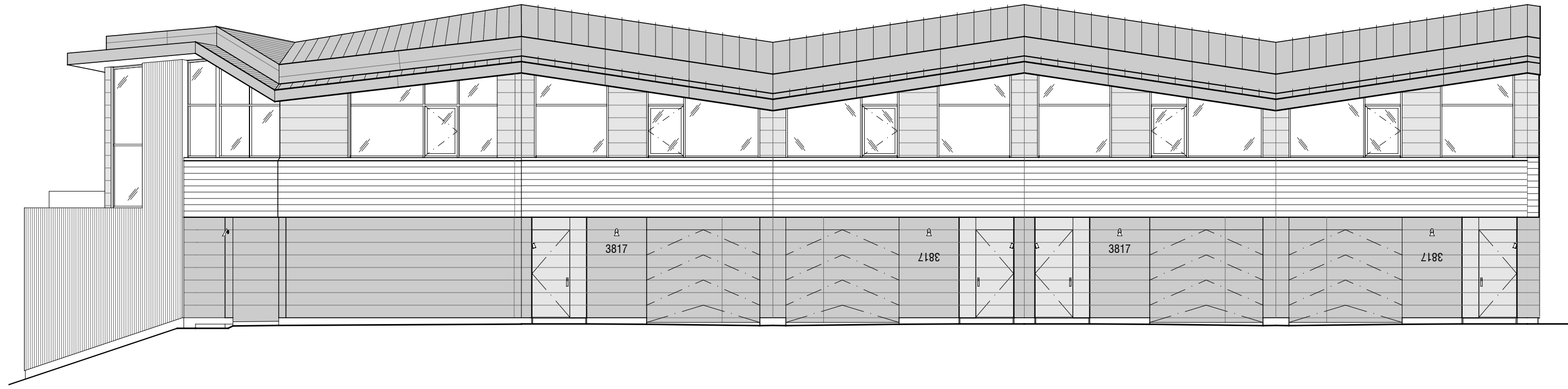
1 OVERALL BUILDING ELEVATION_EAST
