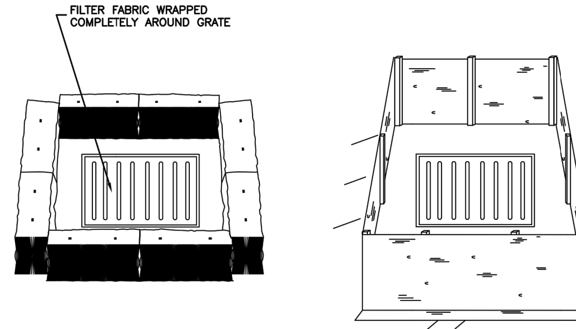
STRAW BALE BARRIER (PLAN No. 121)
