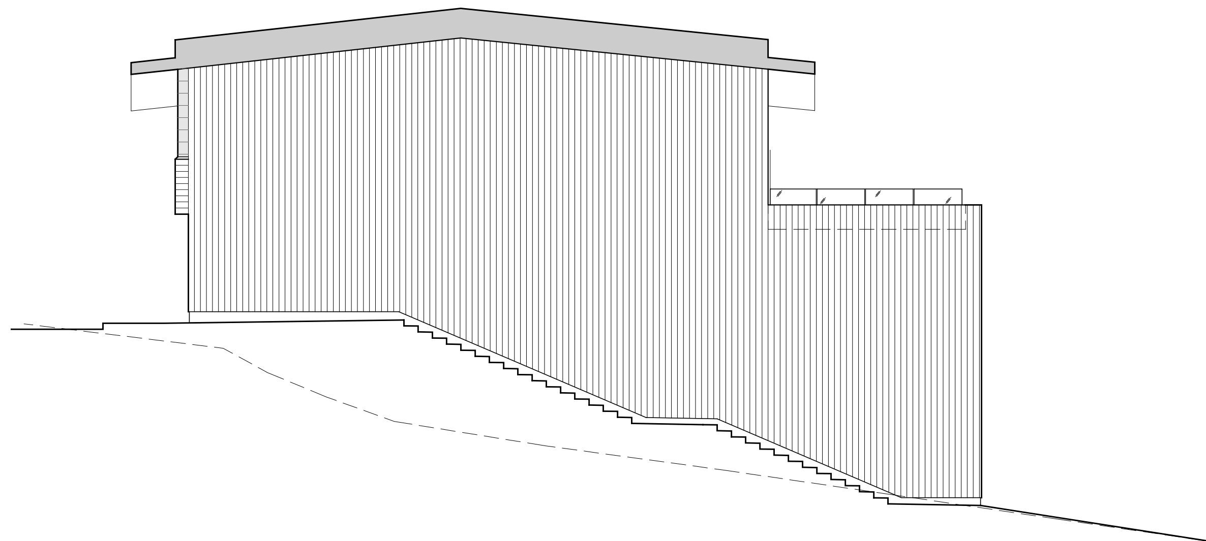
3 OVERALL BUILDING ELEVATION_NORTH
