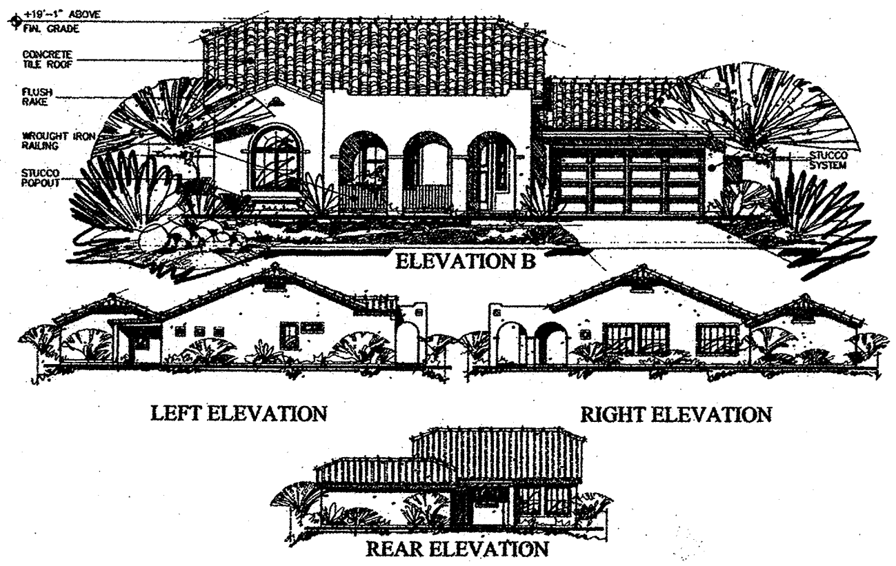
REAR ELEVATION
