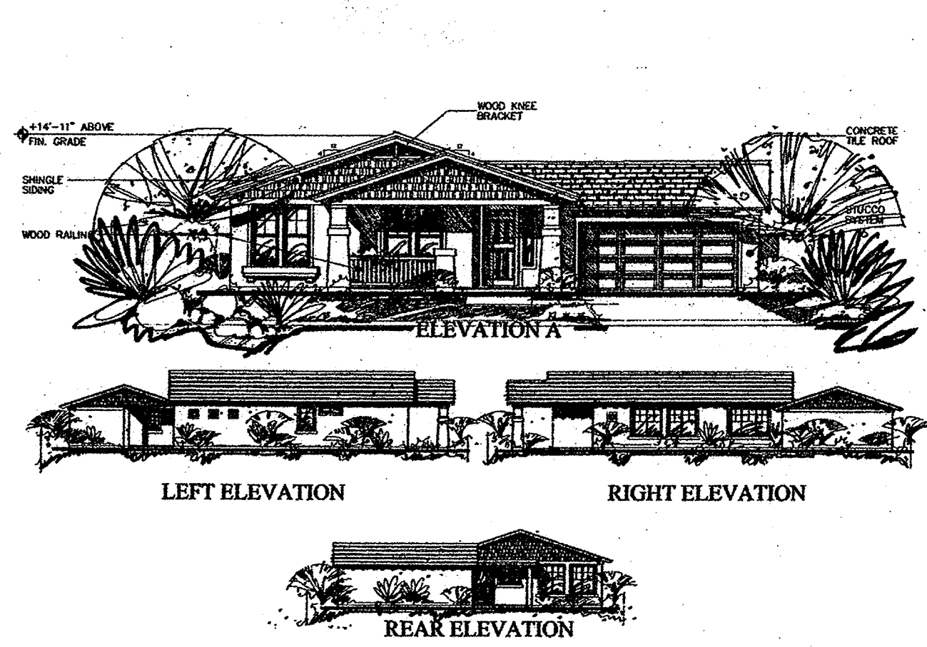
REAR ELEVATION
