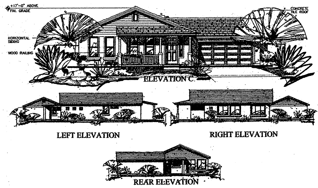
REAR ELEVATION
