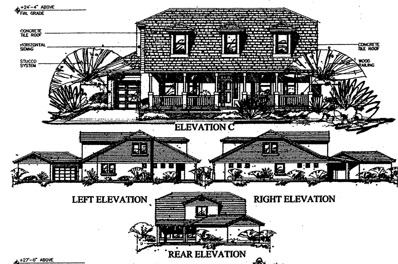
REAR ELEVATION
