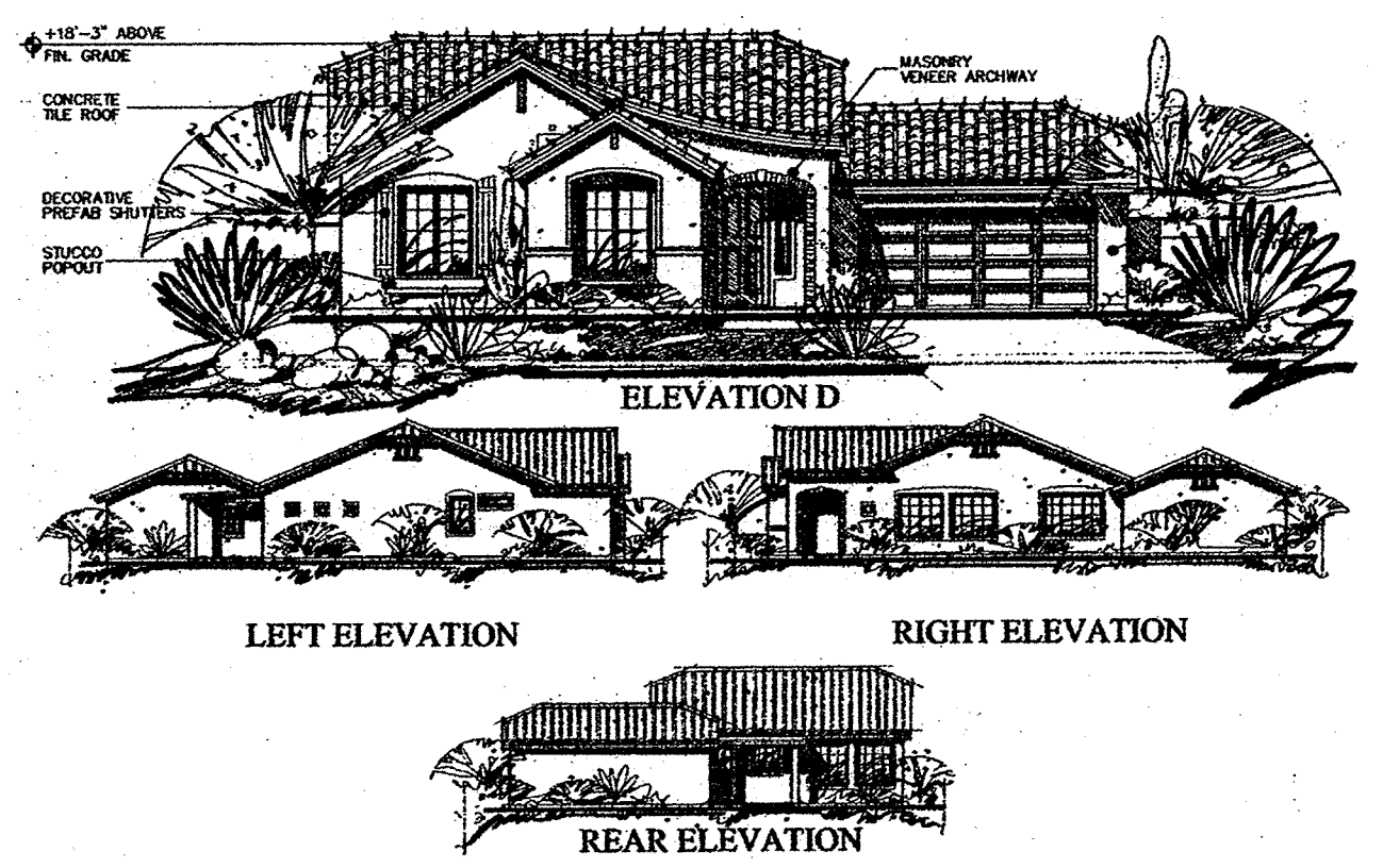
REAR ELEVATION
