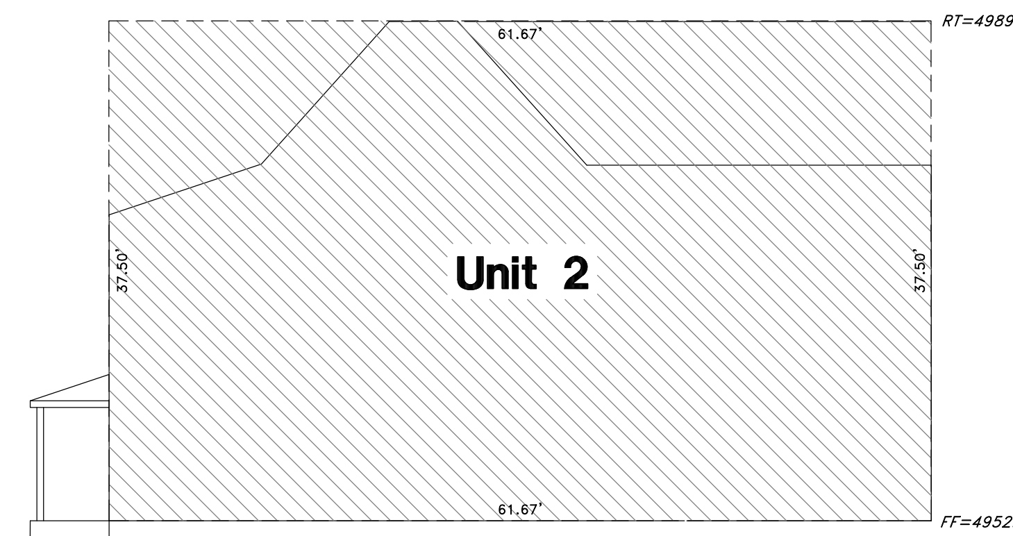
Section BB-BB
