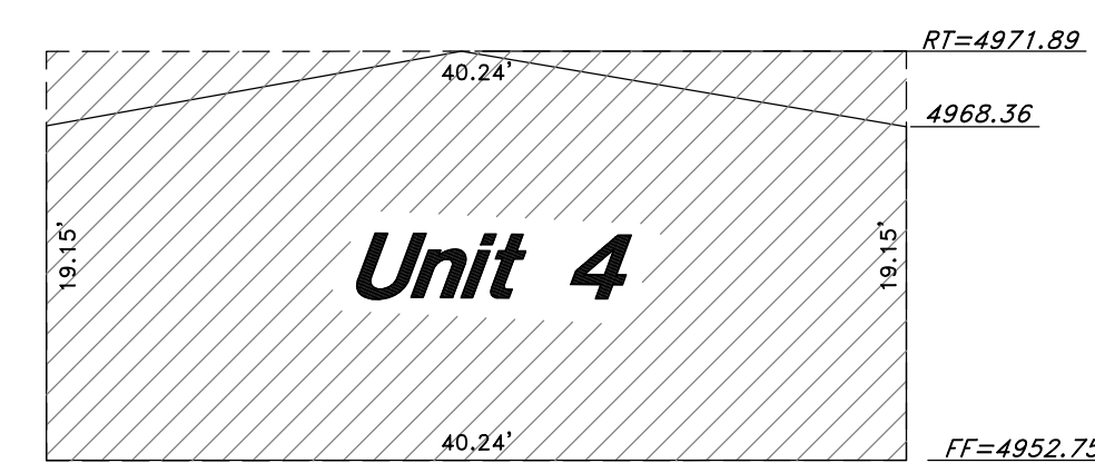
Section DD-DD
