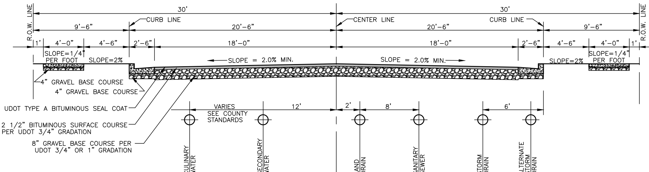
Street Section (60' R.O.W.) SCALE: NONE
