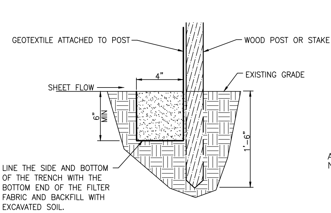
Section
