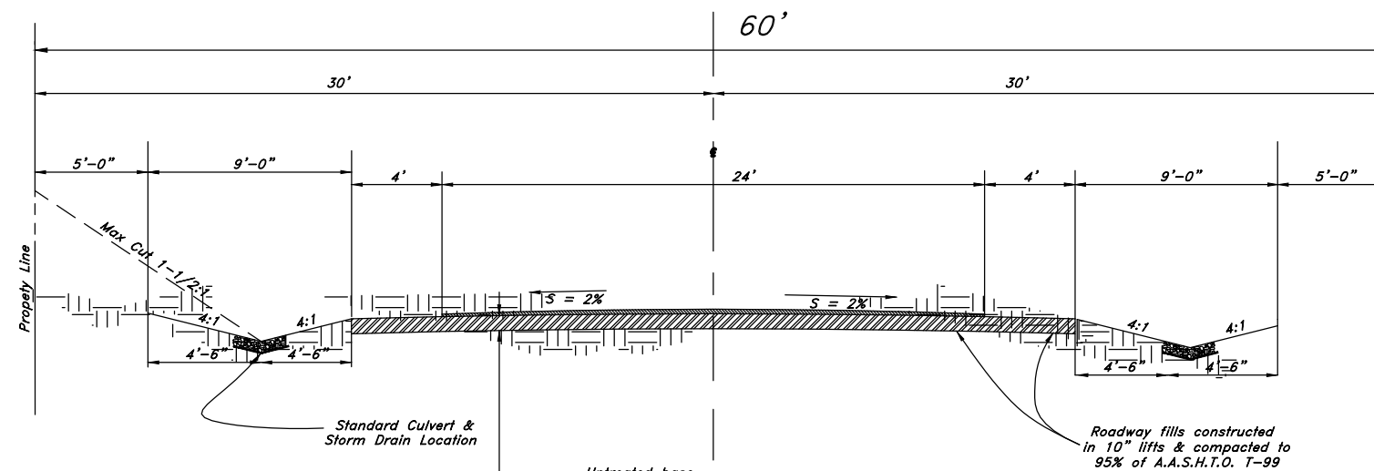
Standard Rural Roadway Section M.I. 8, 2008
