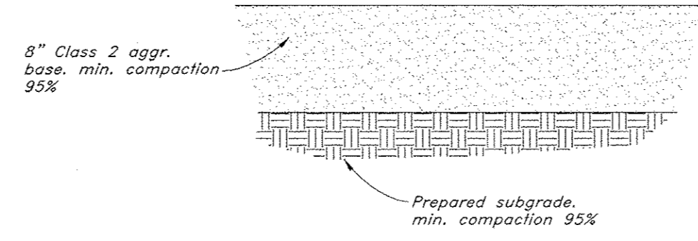
# Typical Gravel Fire Apparatus Turn Around Section Not to Scale
