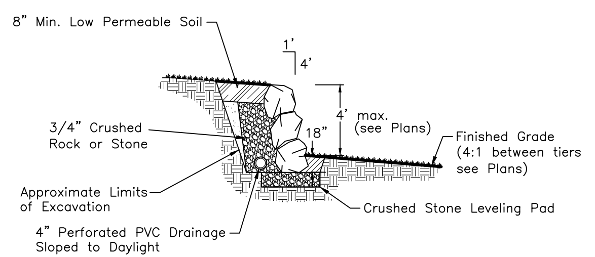
Typical Wall Section
