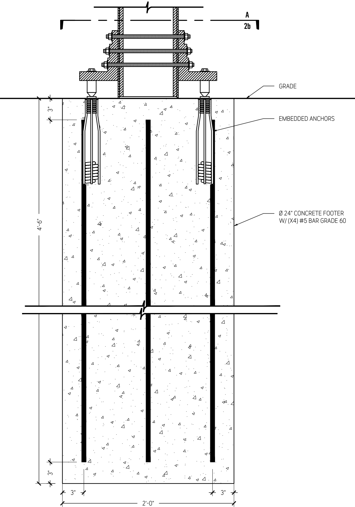
1 FOOTER DETAIL 1 1/2" = 1'-0"
