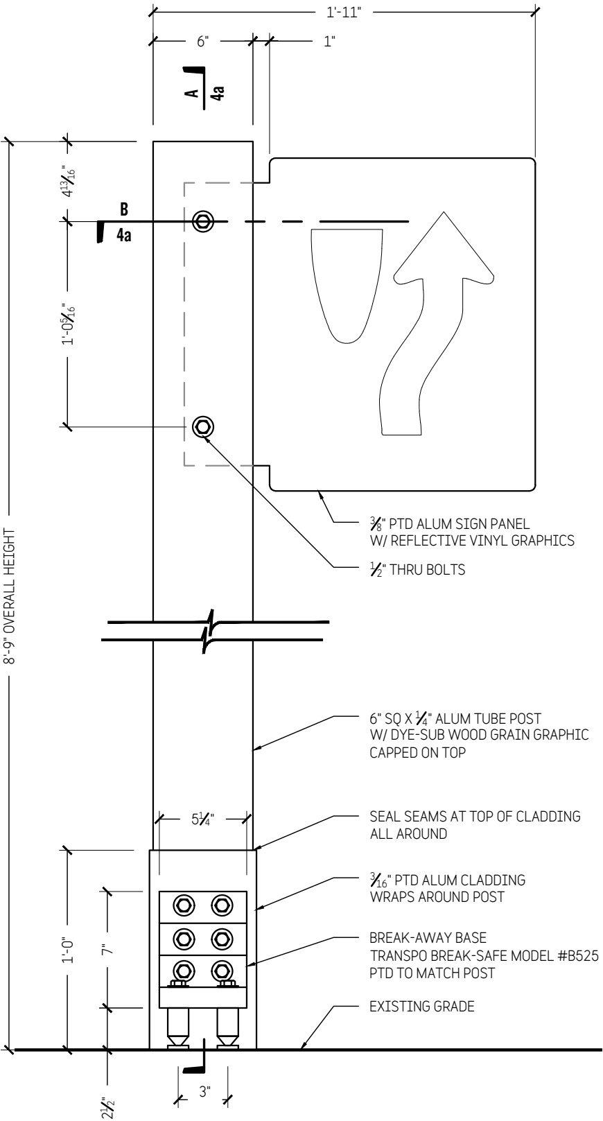
1 FRONT VIEW 1 1/2" = 1'-0"
