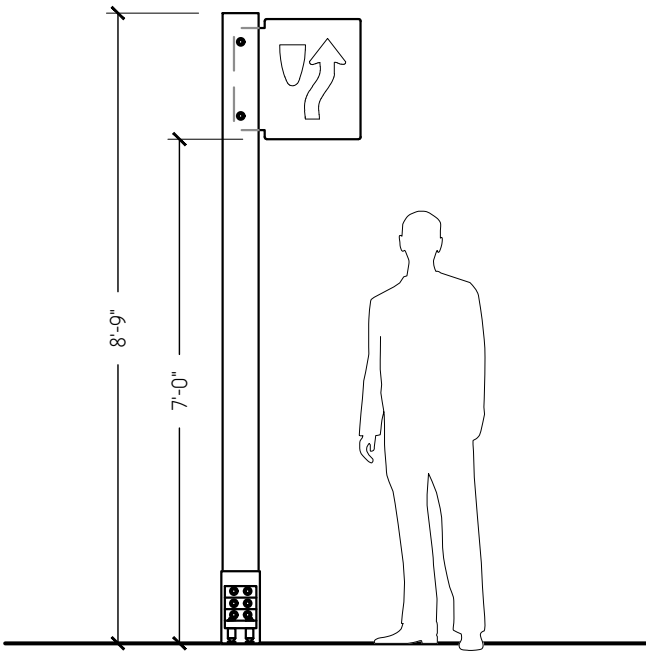
3 ELEVATION 3/8" = 1'-0"
