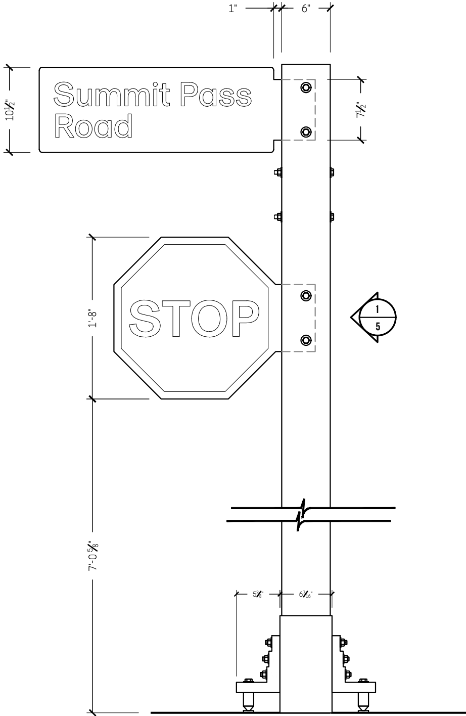
3 ELEVATION 1/4" = 1'-0"
