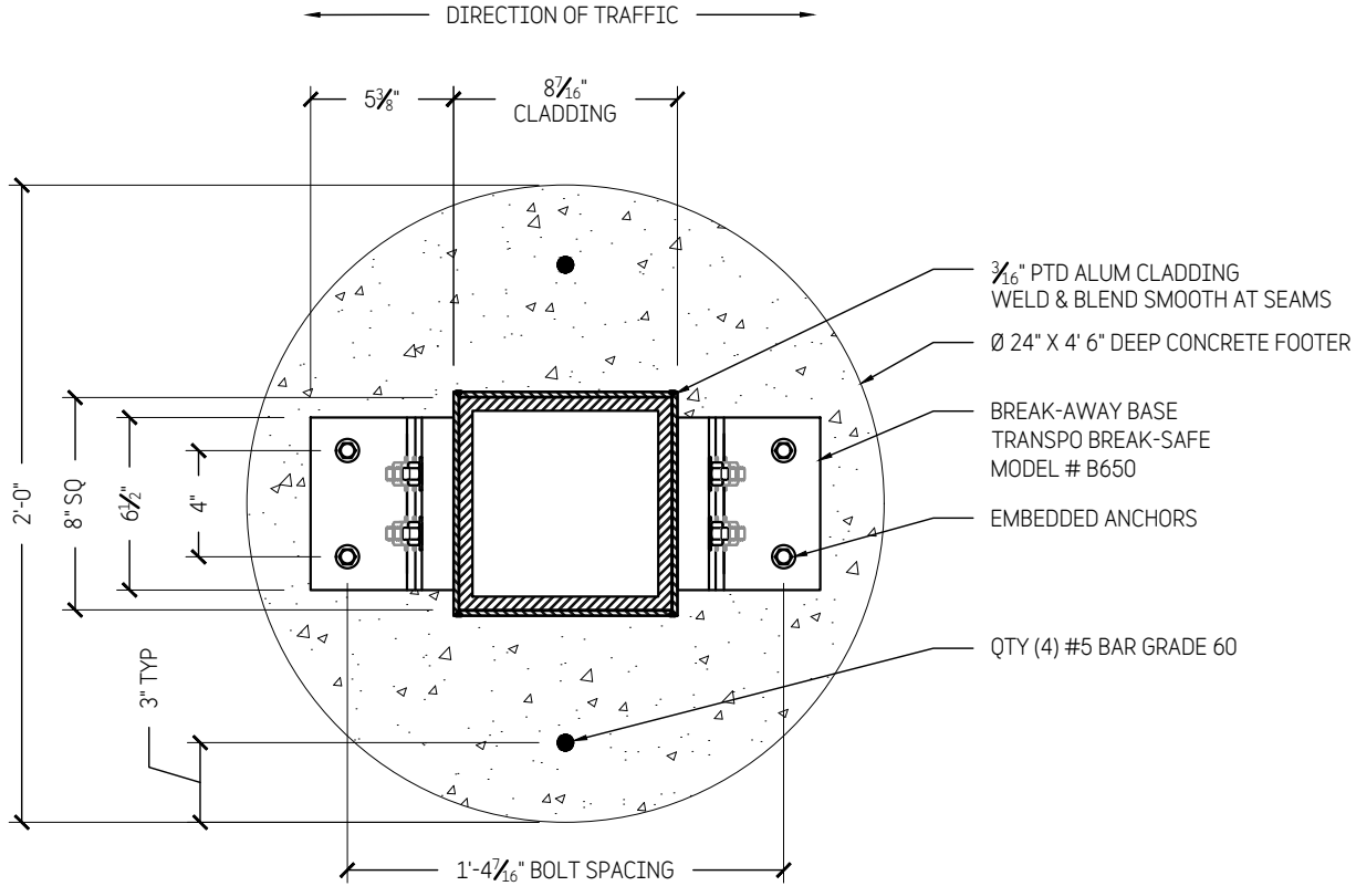
A SECTION 1 1/2" = 1'-0"
