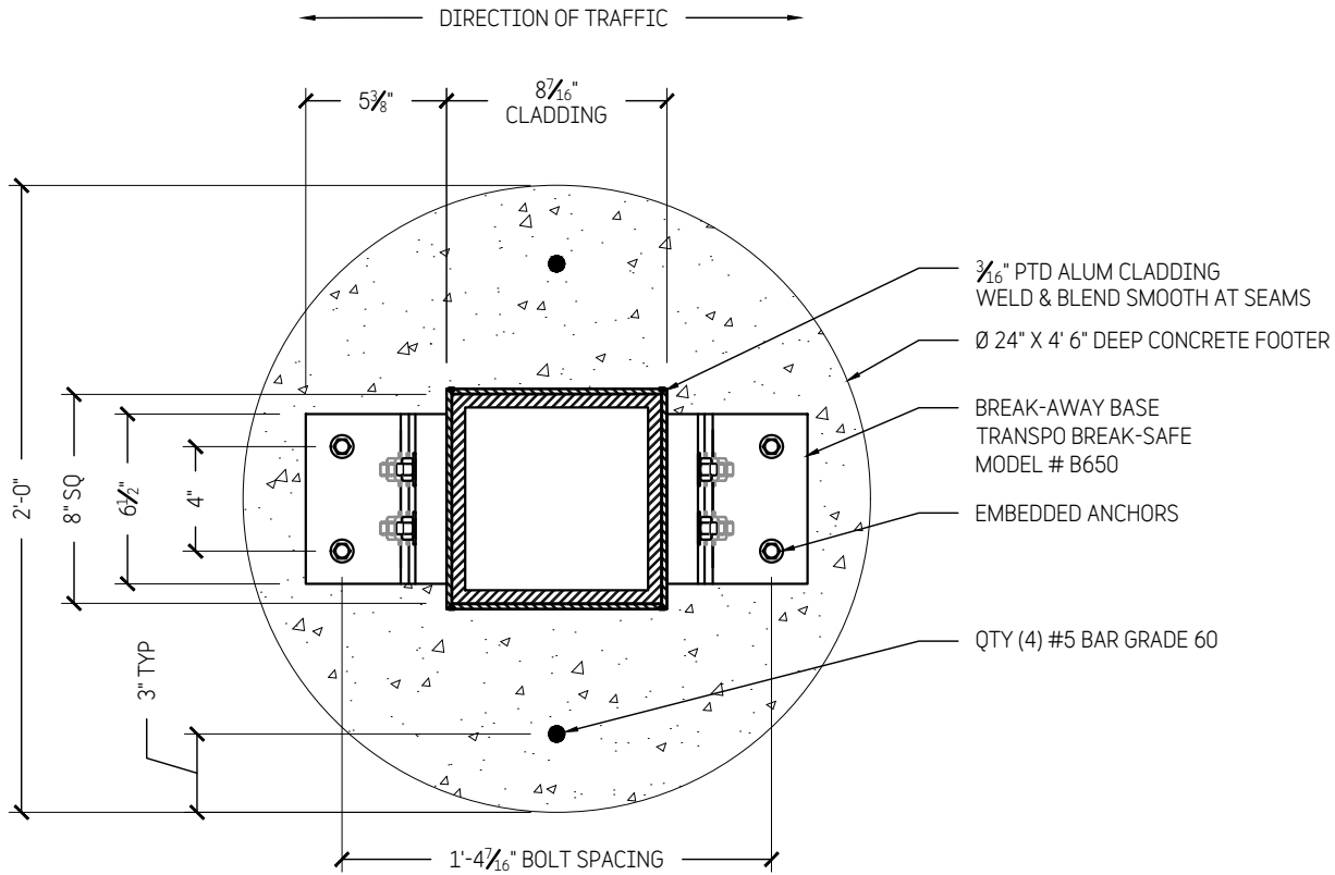
A SECTION 1 1/2" = 1'-0"
