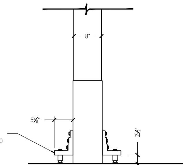
2 SIDE VIEW
