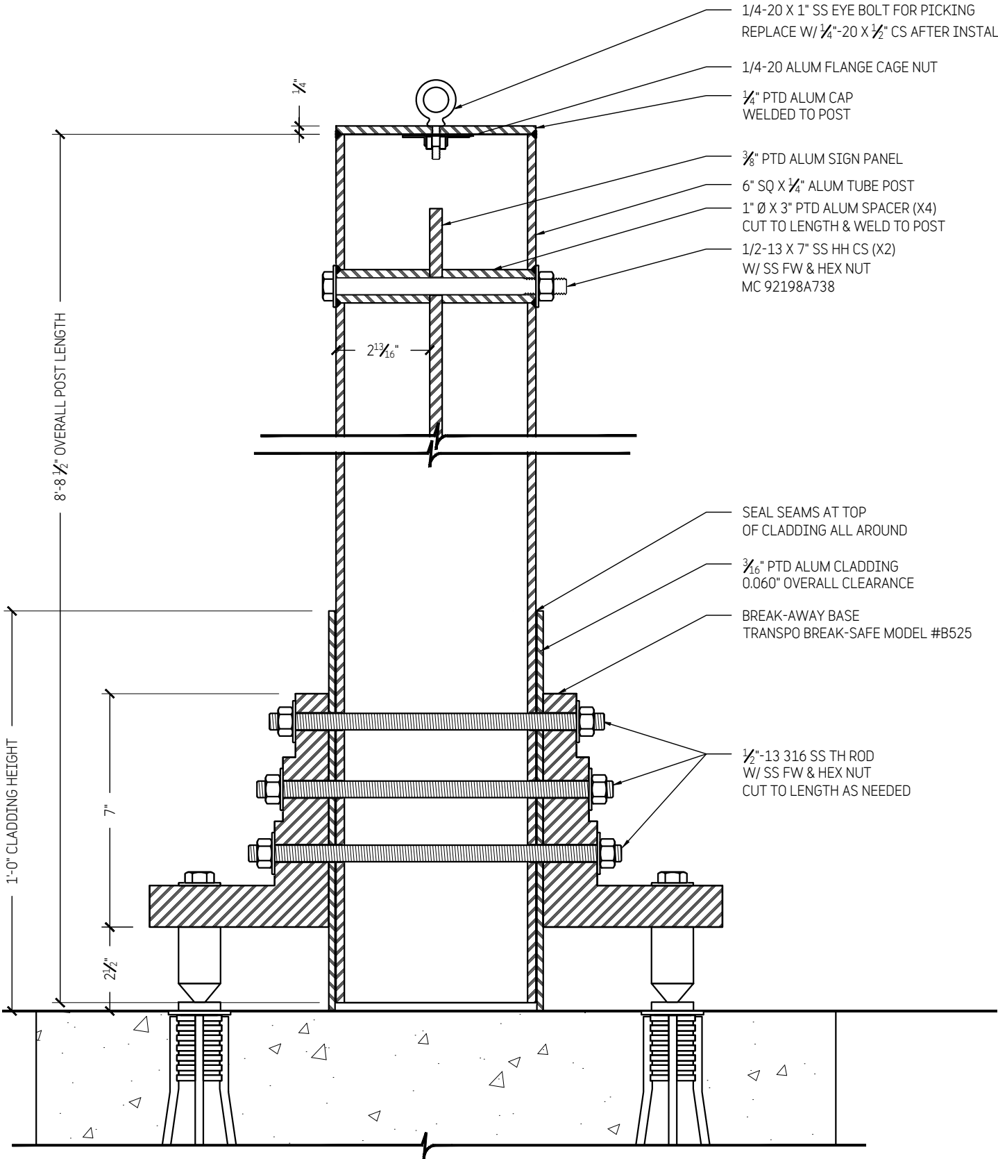
A SECTION 3" = 1'-0"
