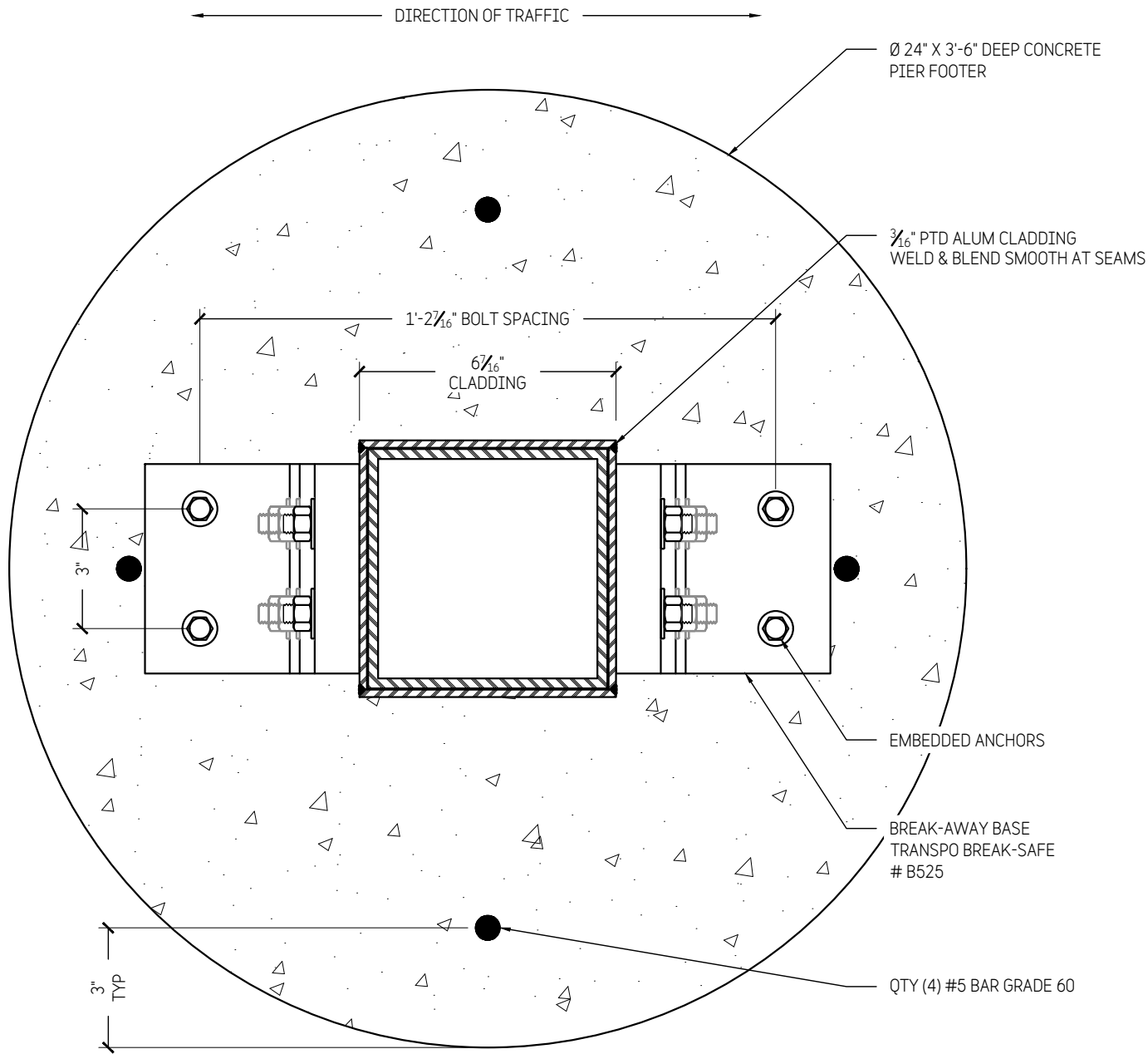
A SECTION 3" = 1'-0"
