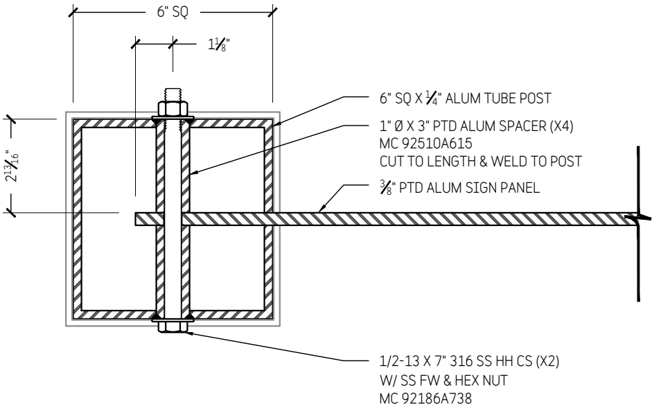
B SECTION 3" = 1'-0"
