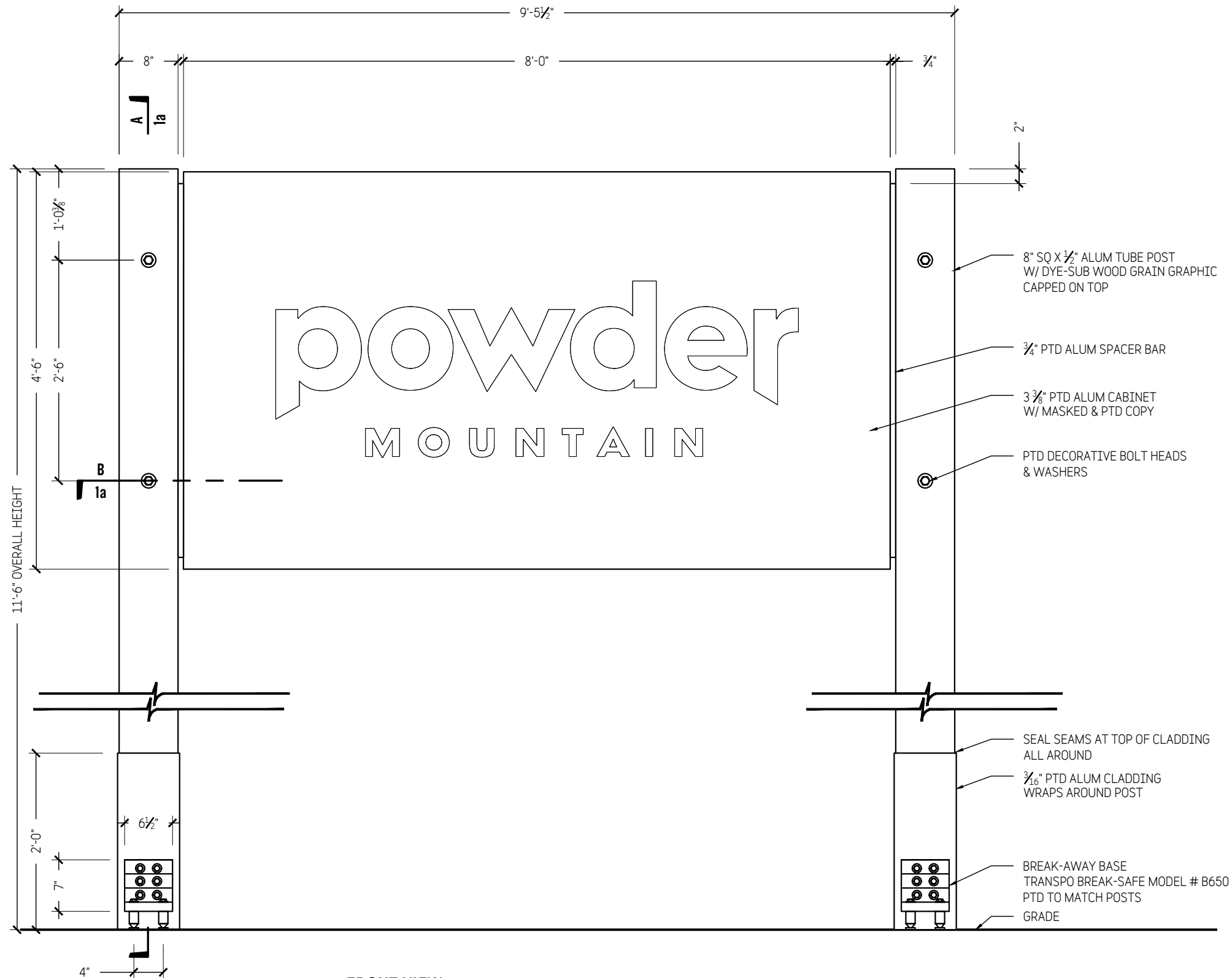
1 FRONT VIEW
