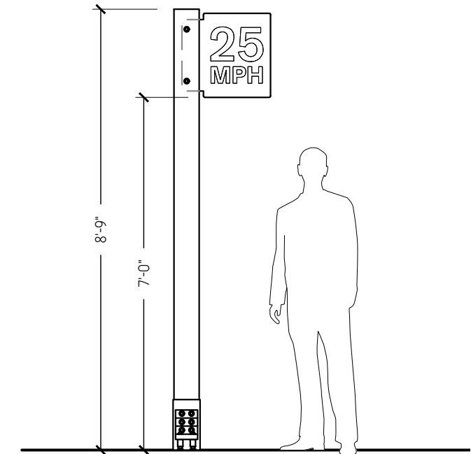
3 ELEVATION 3/8" = 1'-0"
