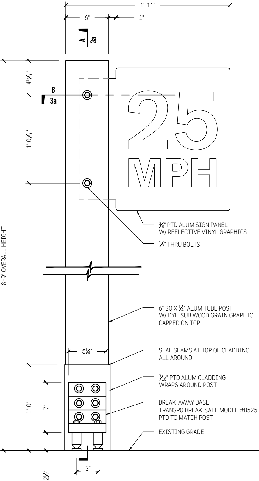
1 FRONT VIEW 1 1/2" = 1'-0" QTY: 4 D/S
