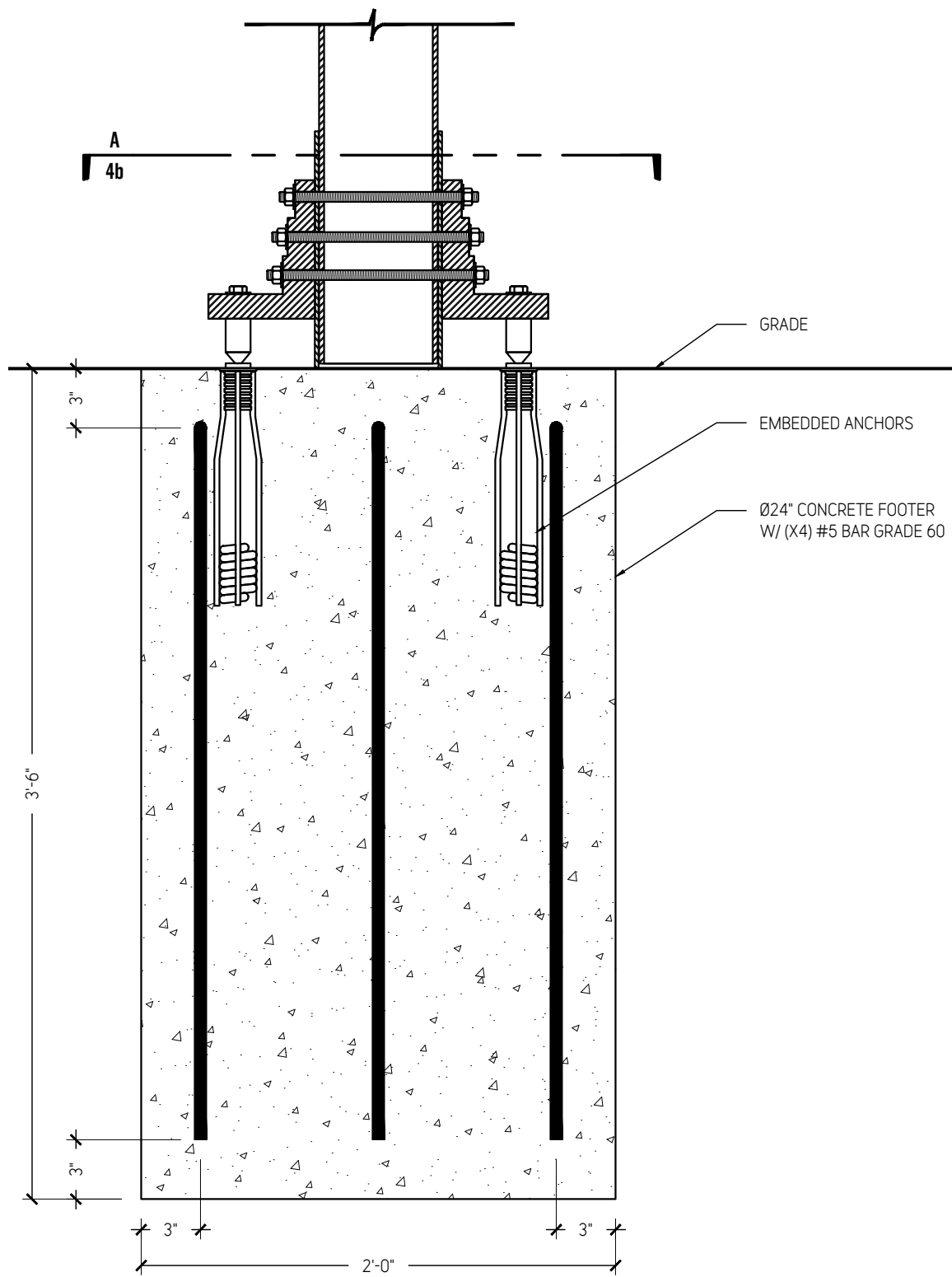
1 FOOTER DETAIL 1 1/2" = 1'-0"
