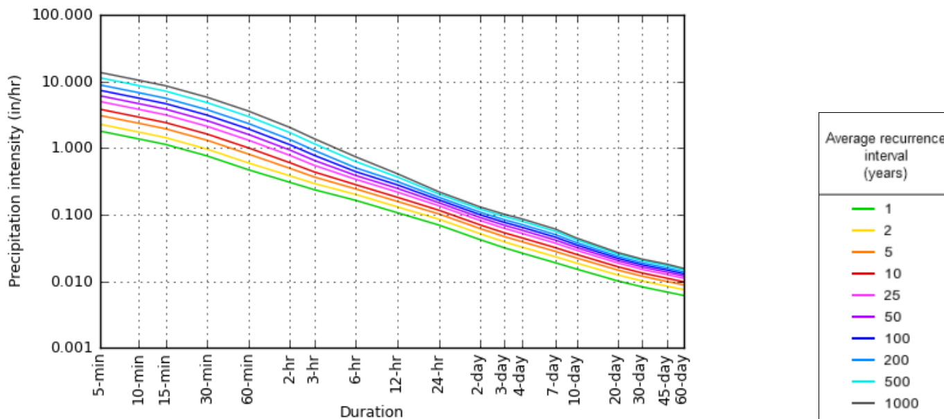
PDS-based intensity-duration-frequency (IDF) curves Latitude: 41.2625°, Longitude: -111.7287°
