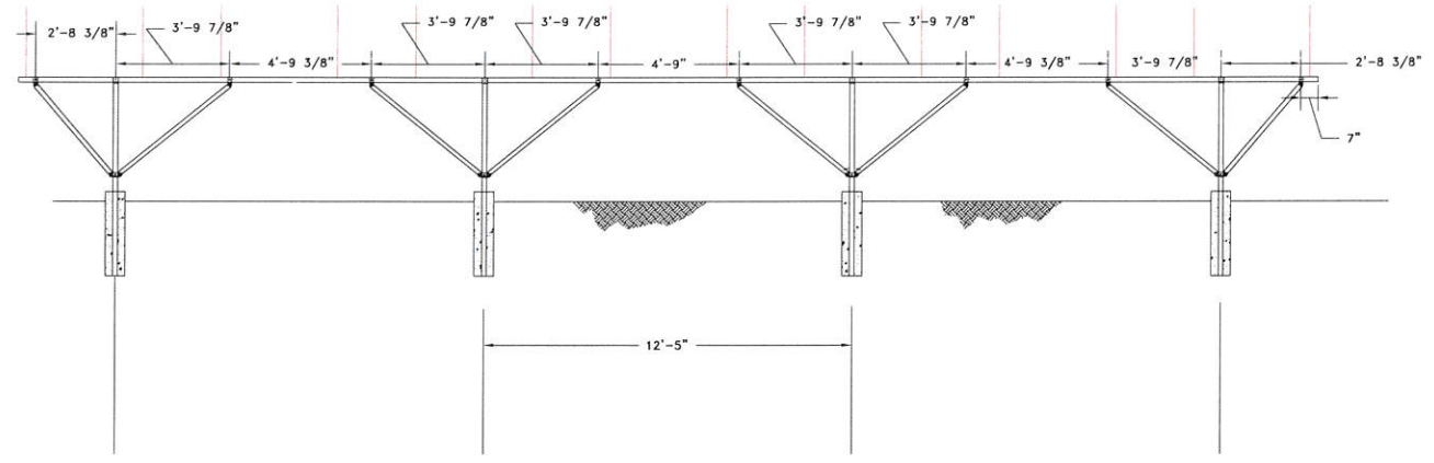
SOUTH - FRONT SUPPORTS
