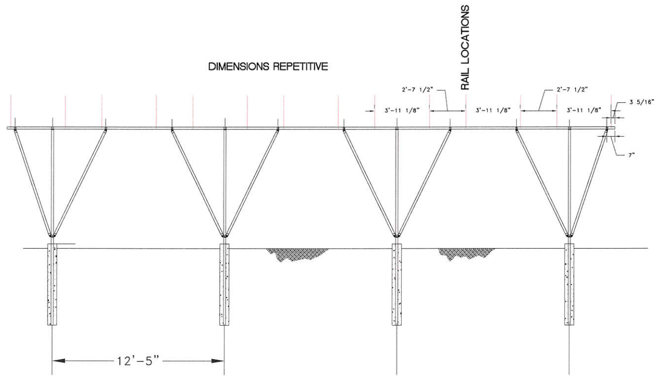
NORTH - REAR SUPPORTS
