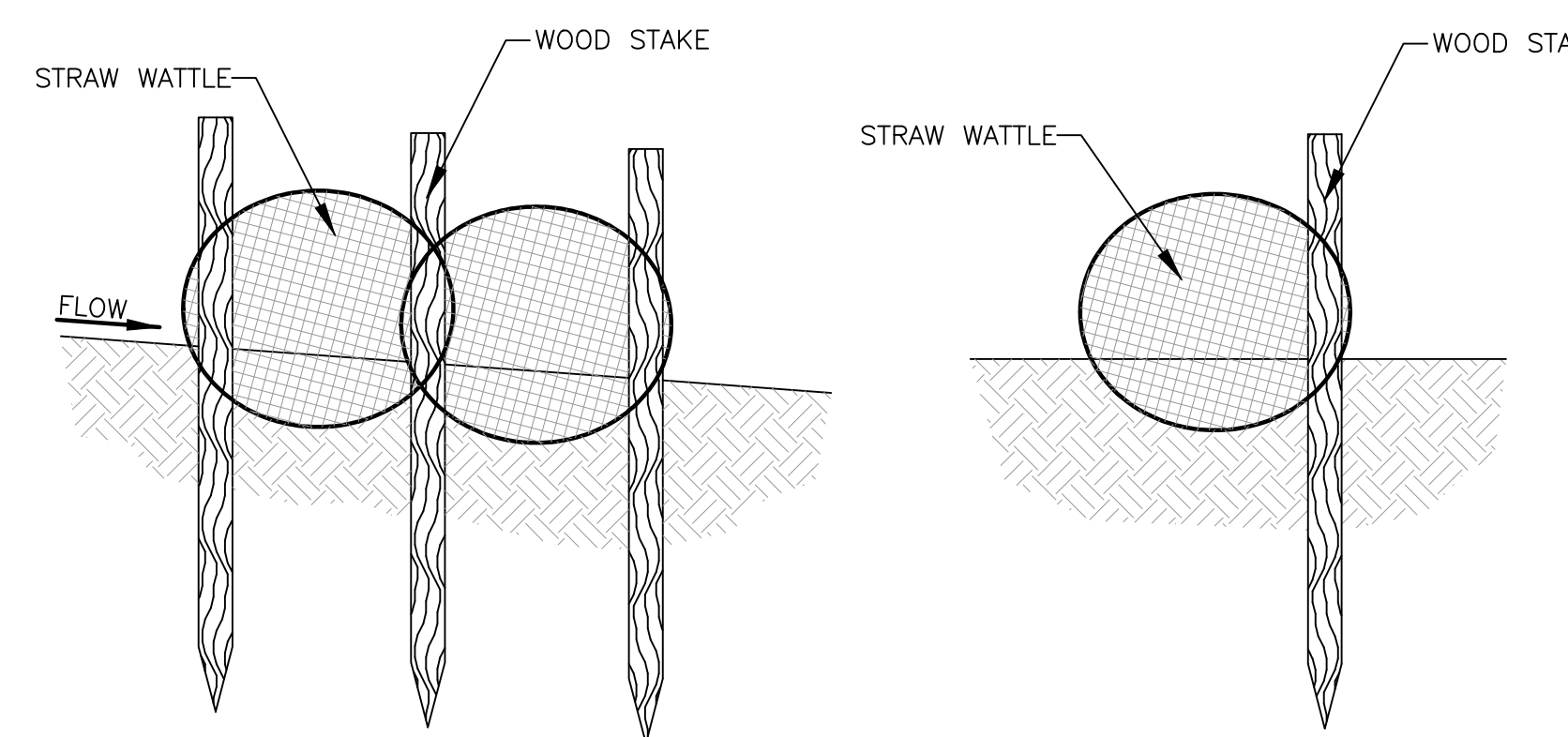
Stake Detail
