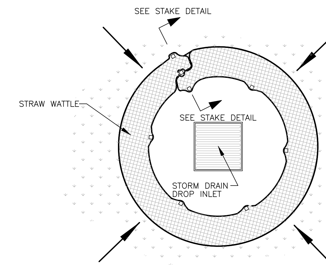
Plan View
