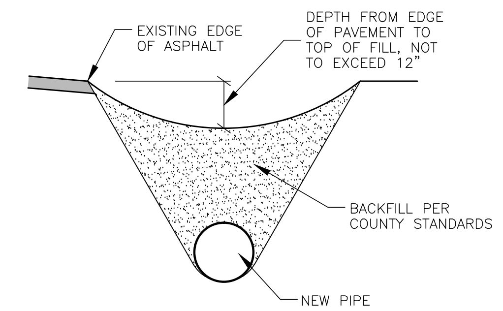
Pipe/Ditch Backfill Detail
